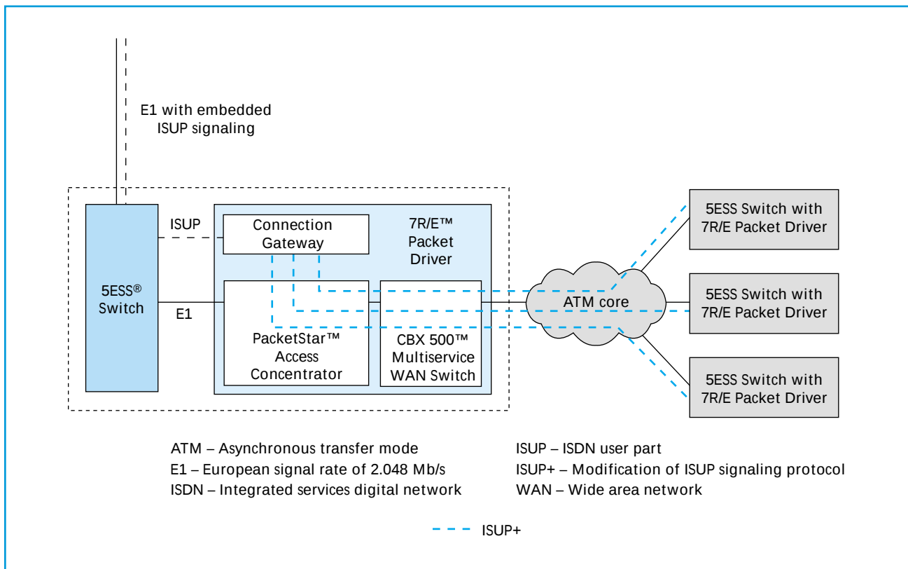
Figure 1. VTOA network architecture.
