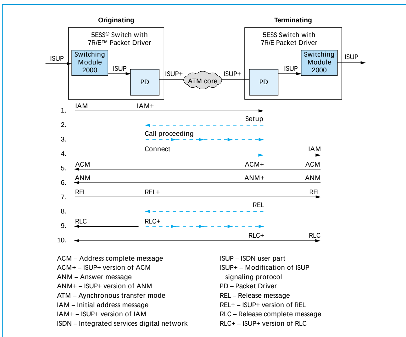
Figure 5. Basic VTOA call scenario using SVCs.
