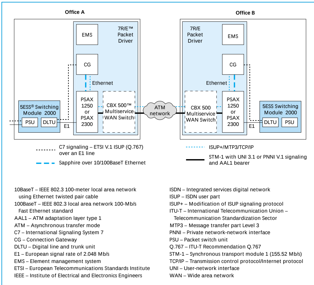
Figure 4. Protocols used for VTOA.
