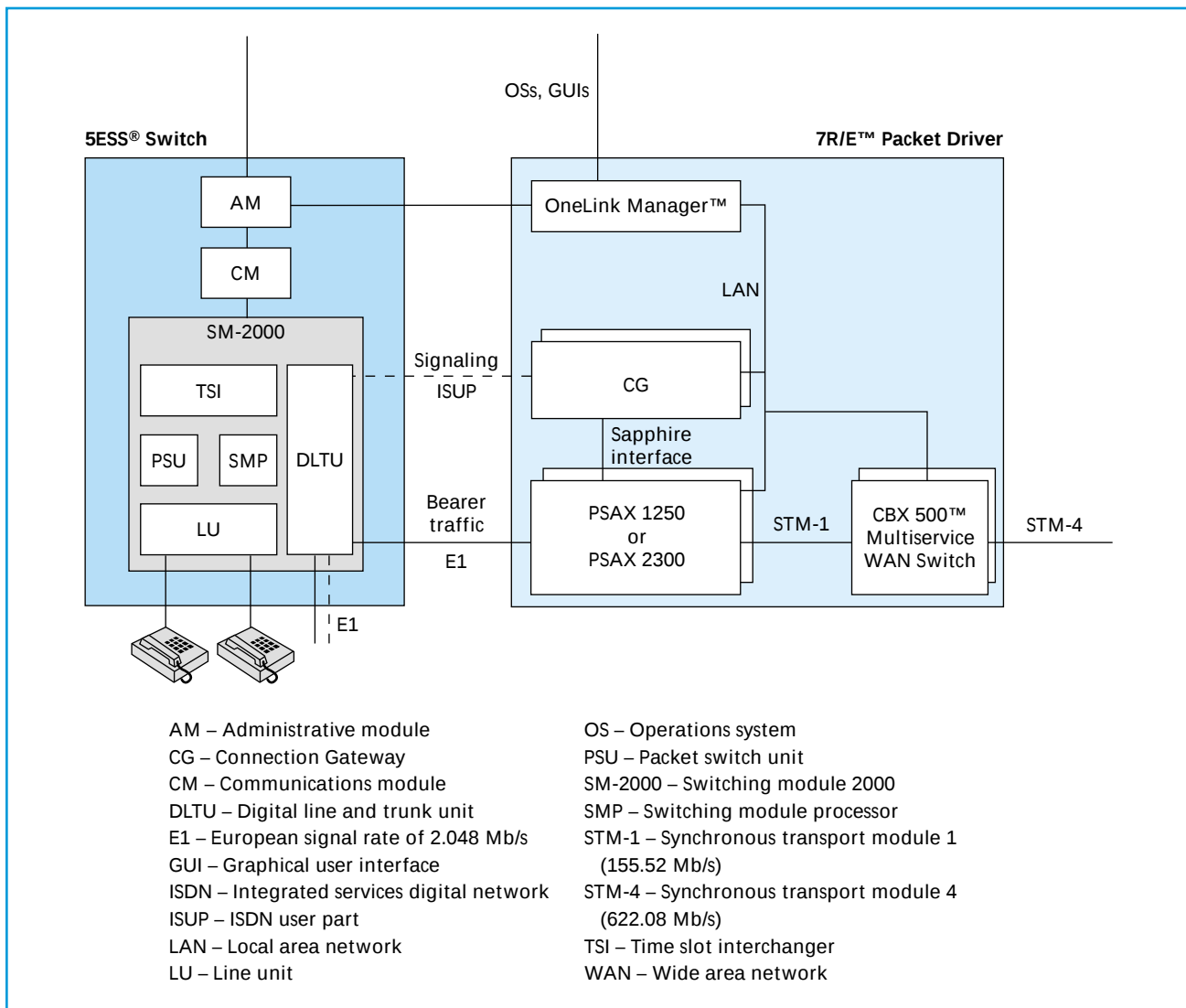
Figure 2. 5ESS® Switch with 7R/E™ Packet Driver block diagram.
