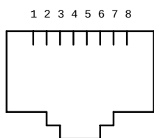
RJ45 Female Jack Front View
