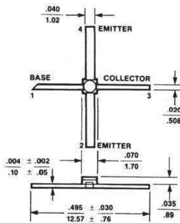
AVANTEK 70 mil PACKAGE
