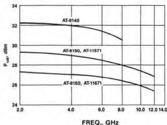
1 dB COMPRESSED GAIN vs. FREQUENCY
