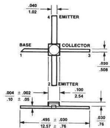
AVANTEK 100 mil PACKAGE
