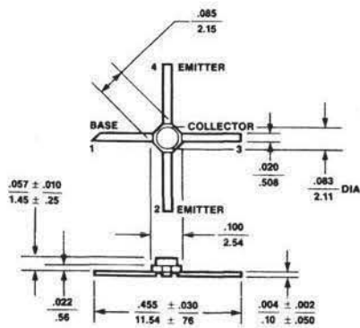
AVANTEK micro-X PACKAGE
