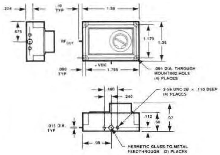
PIN PACKAGE
