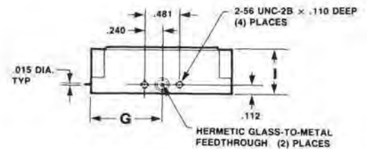
PIN PACKAGE
