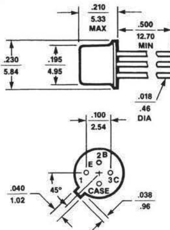
AVANTEK TO-72 PACKAGE
