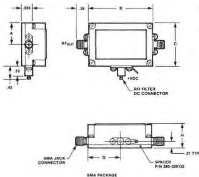
SMA PACKAGE
