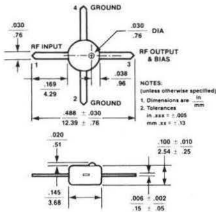
AVANTEK 04 PLASTIC PACKAGE
