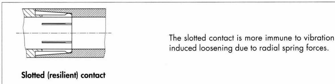
Figure 47 Slotted outer conductor
