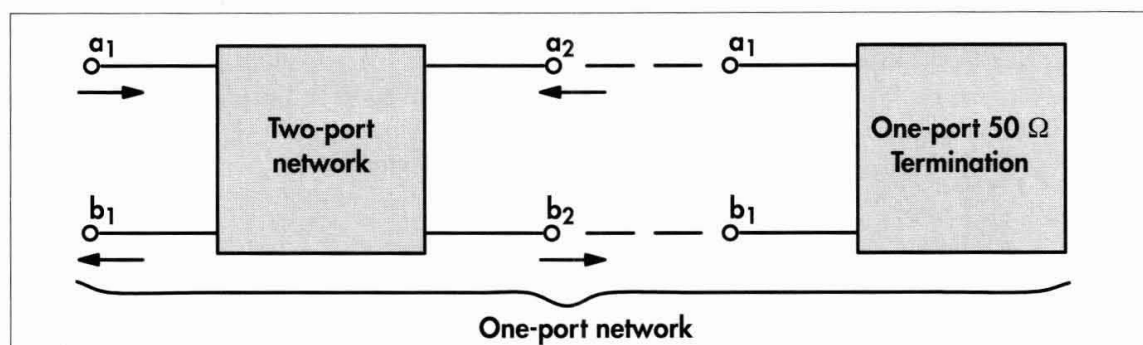
Figure 83 Schematic diagram of one-port network set-up with DUT and 50\ \Omega termination
