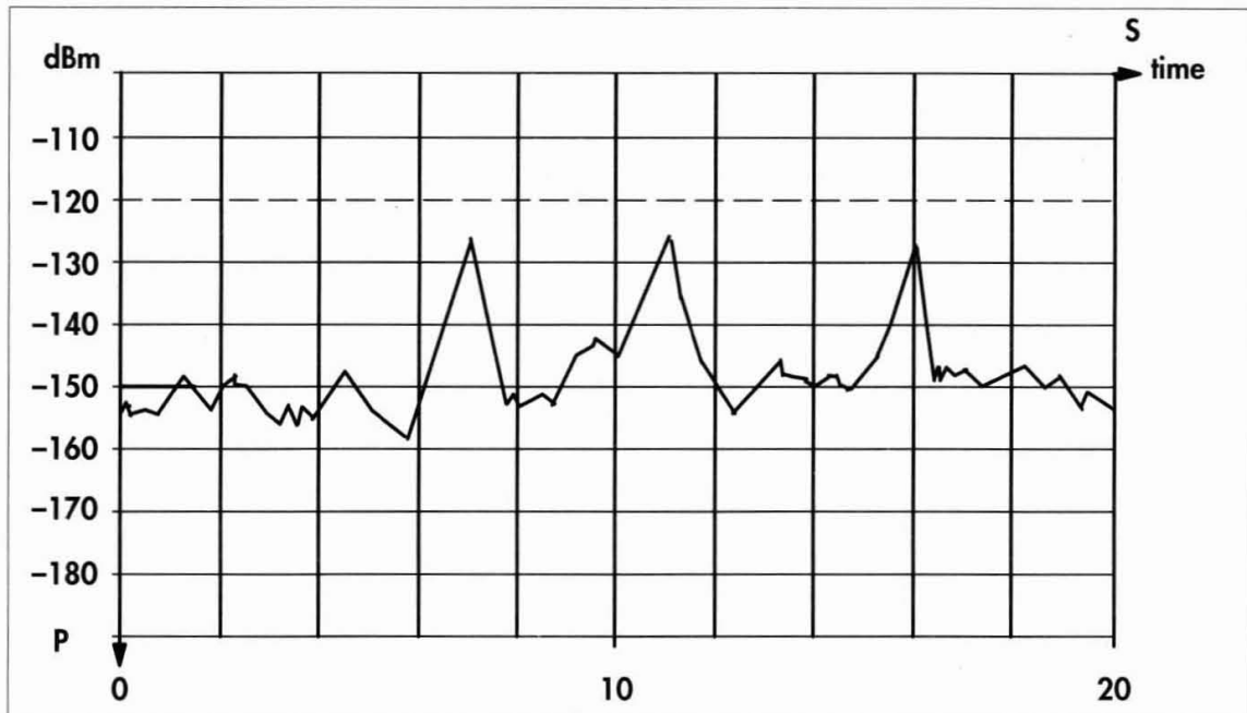
Figure 94 Result of PIM measurement – related to time (time domain in seconds)
