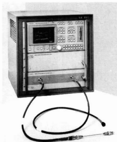
Figure 89 Photograph of test set-up No. 2 with N assembly
