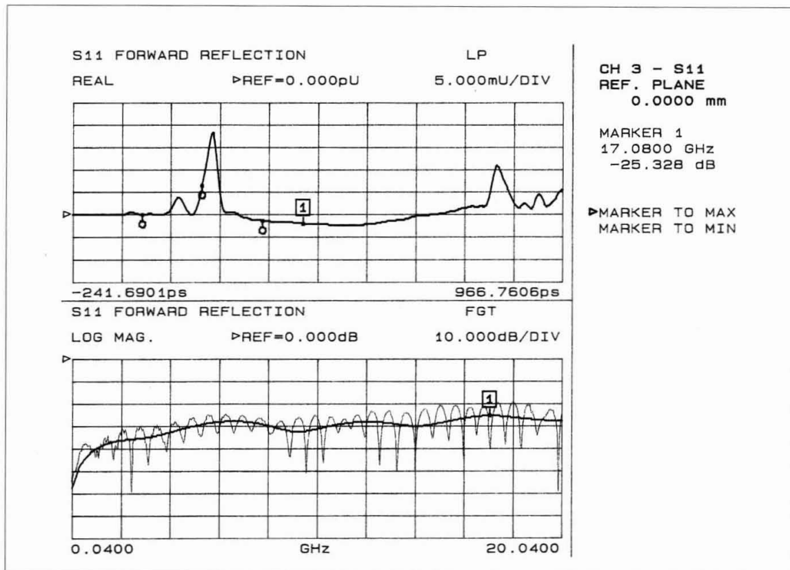
Figure 90 Result of the test No. 2 – related to time (pico-seconds) and frequency
