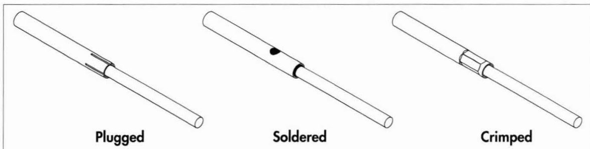
Figure 55 Attachments of the inner conductor
