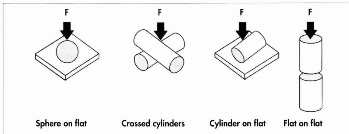
Figure 38 Contact geometry
