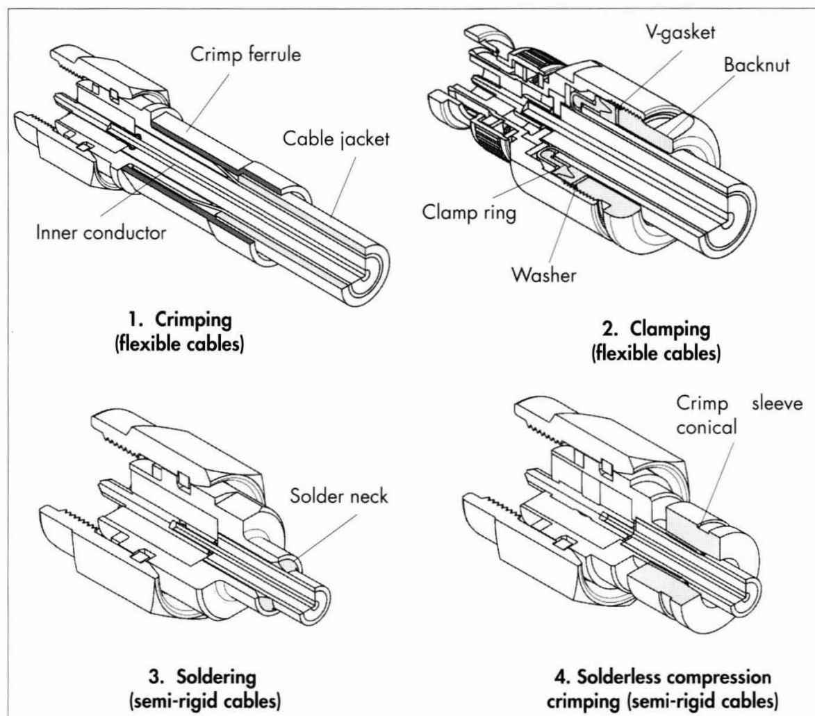
Figure 56 Attachments of the outer conductor
