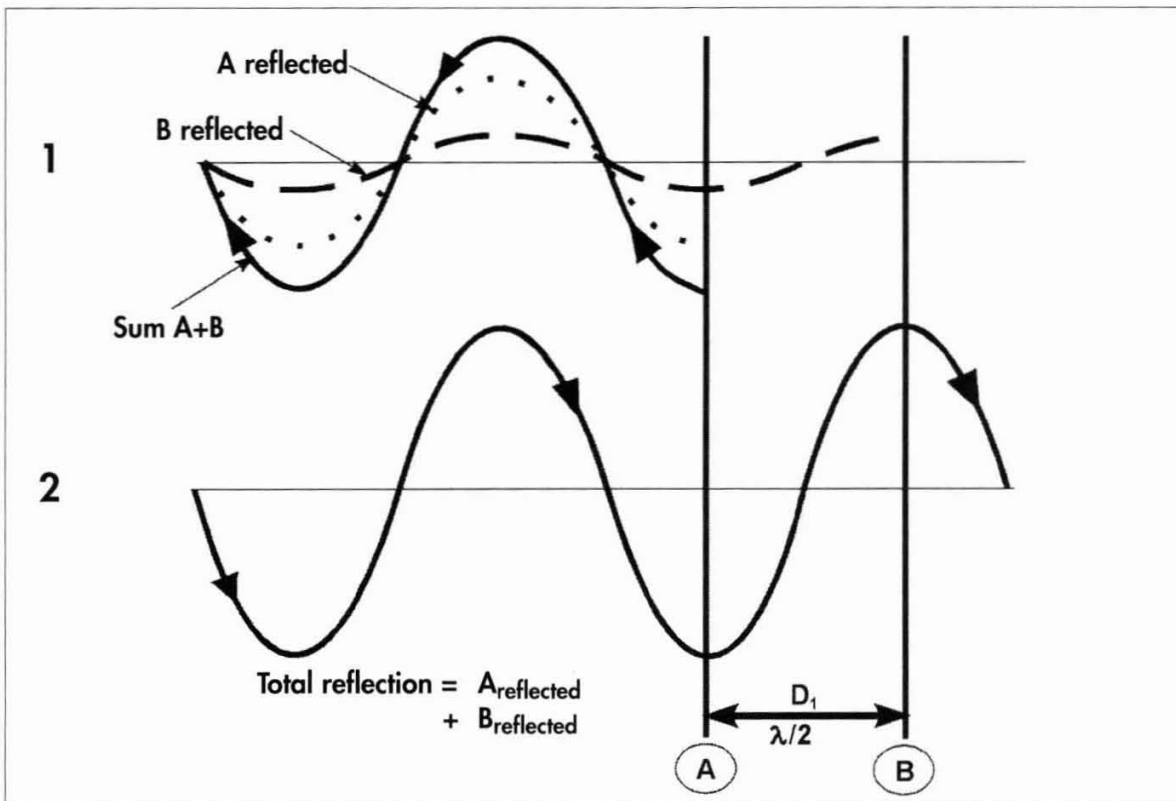
Figure 28 Two reflected waves (1) equivalent to total reflection (2)
