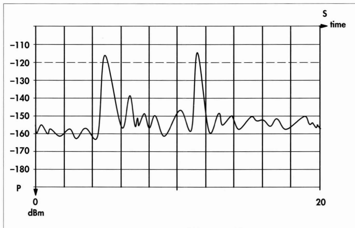
Figure 96 PIM levels after environmental tests and 2 taps – in time domain
