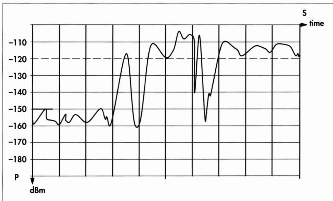
Figure 97 Unstable PIM behaviour after a tap test
