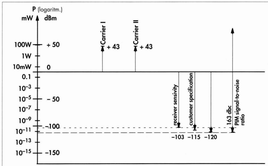
Figure 95 Power relations in the PIM measurement example
