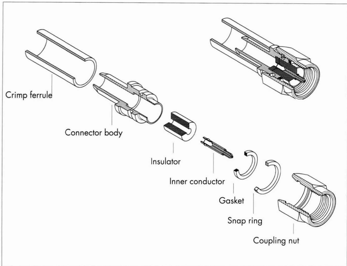
Figure 42 Connector components
