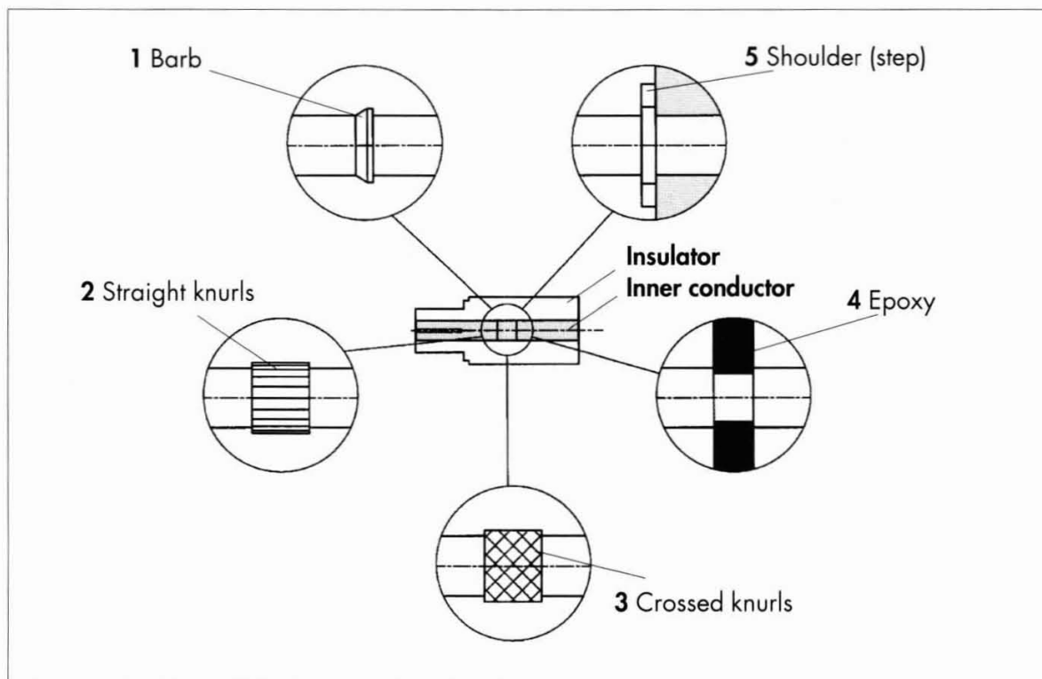
Figure 49 Various inner conductor captivation techniques
