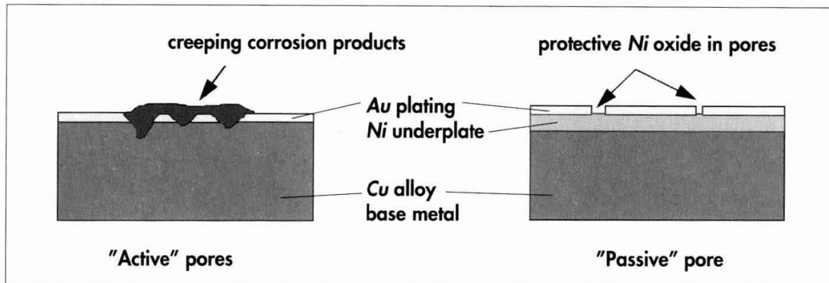
Figure 41 Pore corrosion – microscopical view
