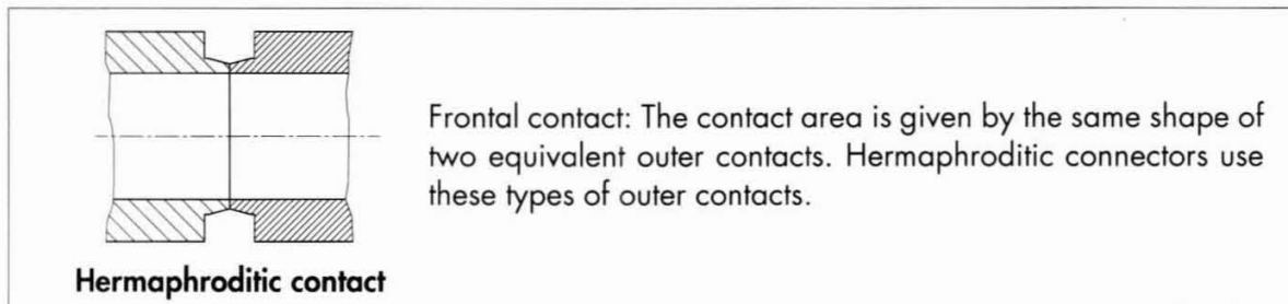
Figure 45 Hermaphroditic (frontally bonded) outer conductor
