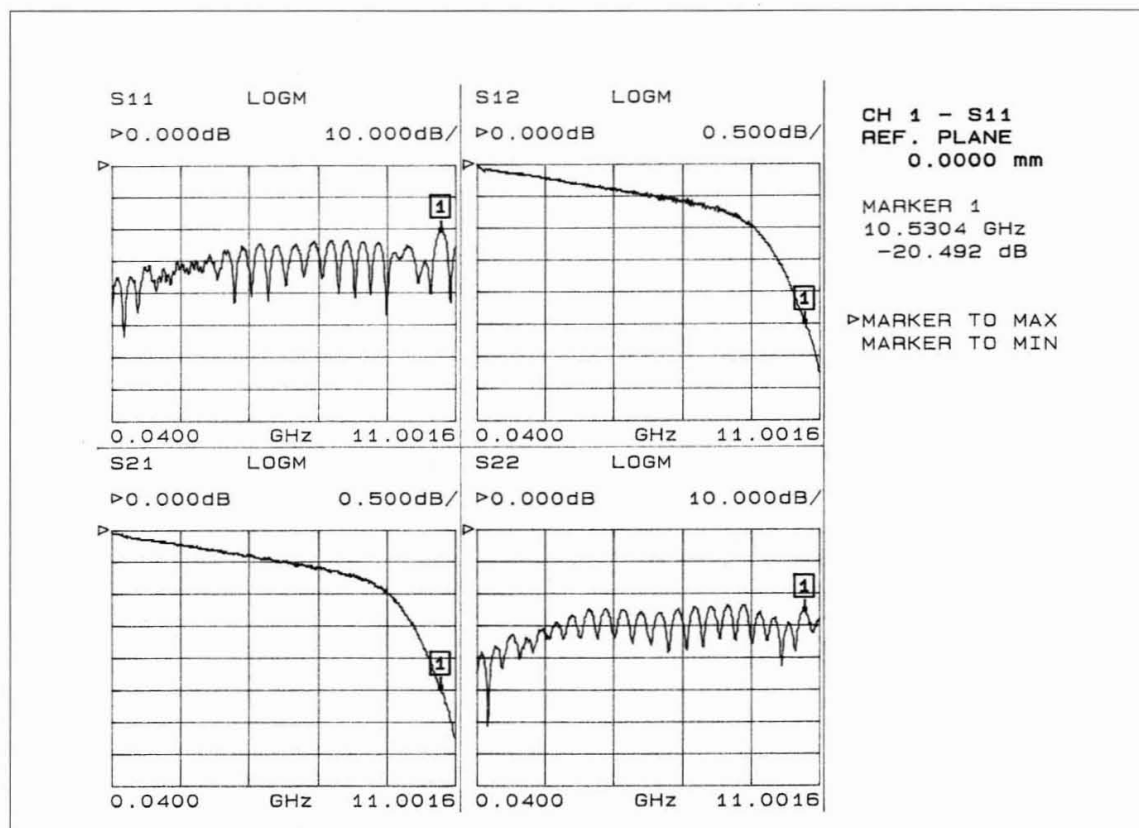
Figure 87 Result of test No. 1 – related to frequency
