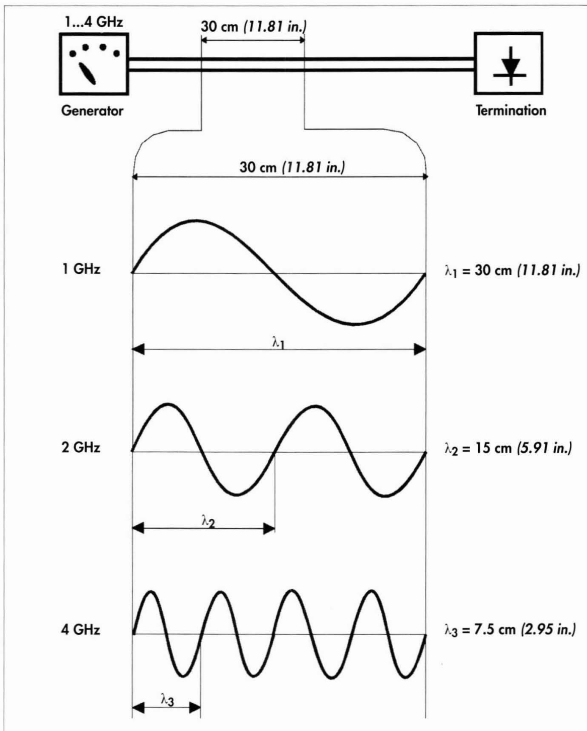
Figure 15 Frequency and wavelength
