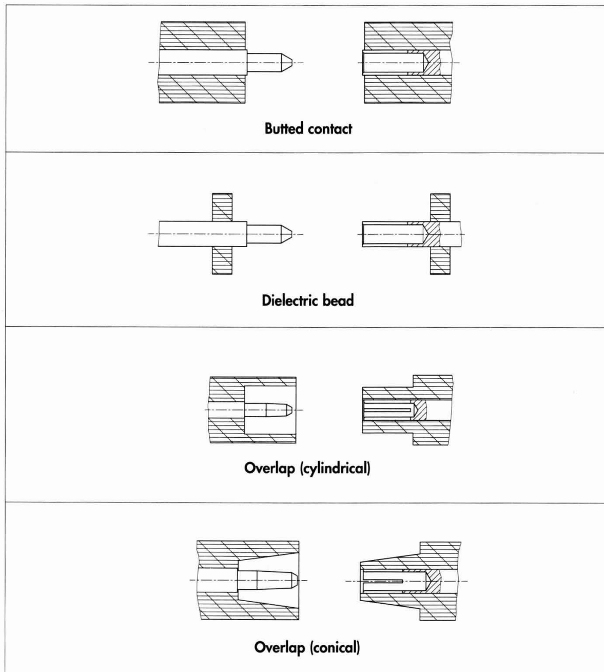
Figure 48 Butt, overlap (cylindrical and conical) and dielectric bead contact
