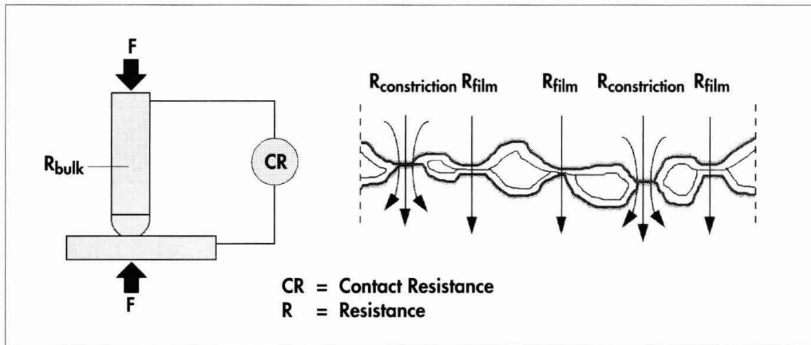
Figure 39 Contact resistance
