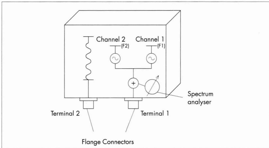
Figure 84 Simplified view of PIM test set-up
