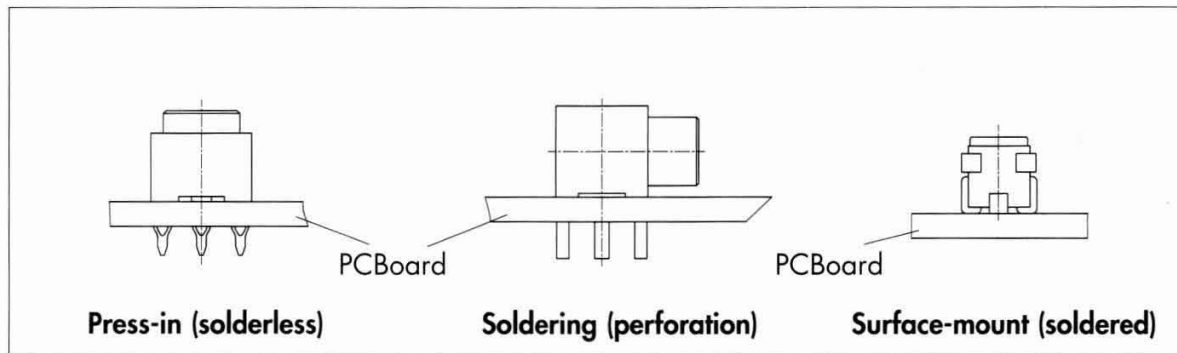
Figure 58 Attachments to a PCB or panel
