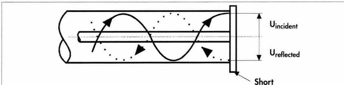
Figure 18 Short circuit
