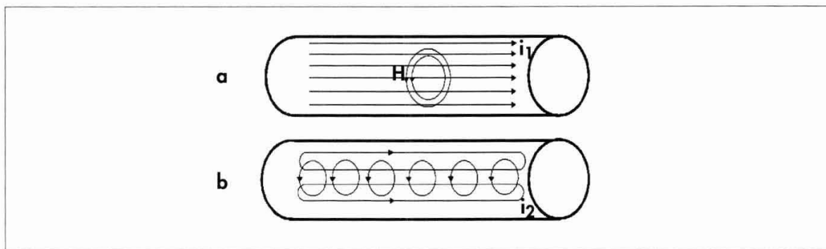
Figure 36 Current density nearing the surface
