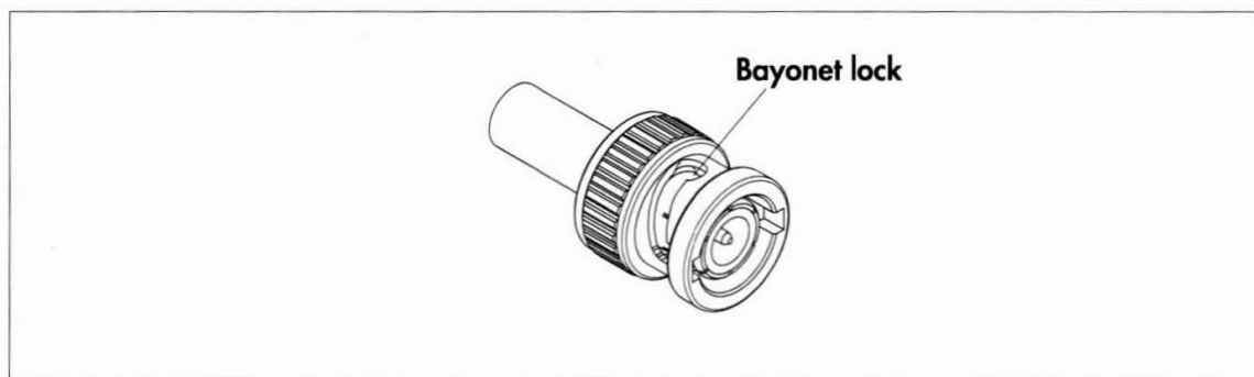
Figure 68 BNC plug connector
