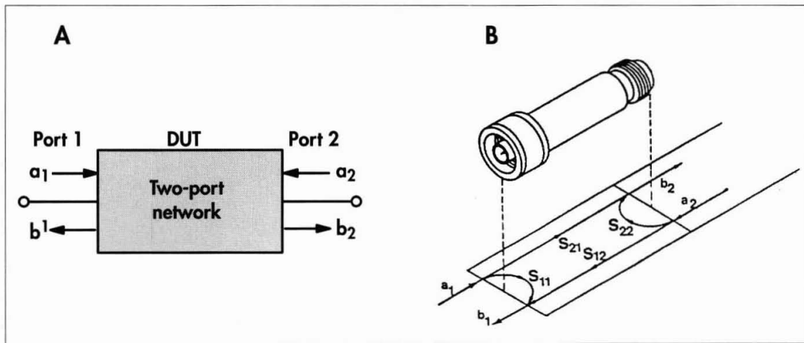
Figure 82 Simplified views of the incoming and outgoing waves in a two-port network
