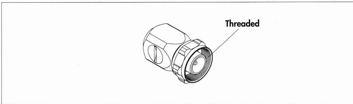
Figure 78 4.1/9.5 plug connector
