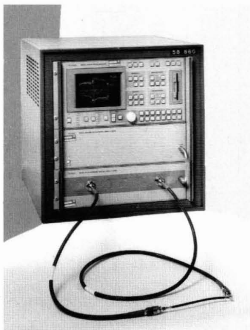
Figure 86 Photograph of test set-up No. 1 with SMA assembly
