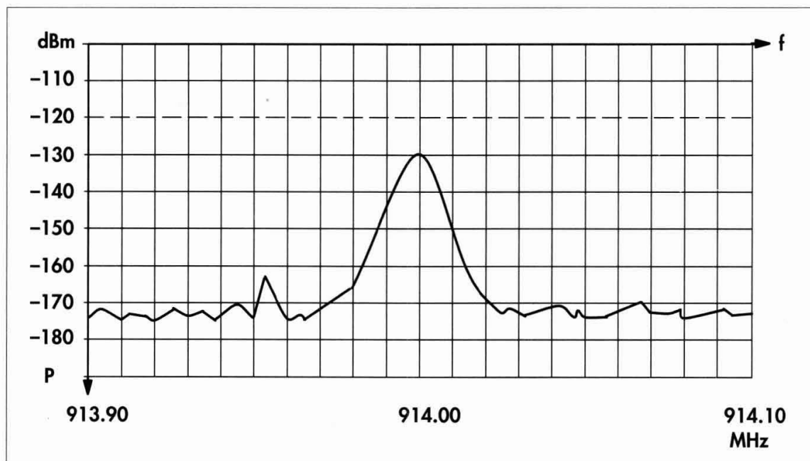
Figure 93 Result of the PIM measurement – related to frequency
