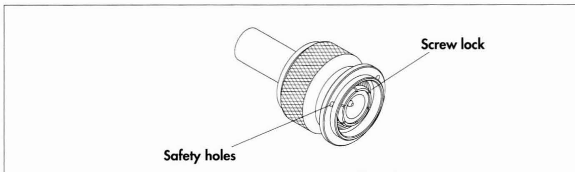
Figure 69 TNC plug connector
