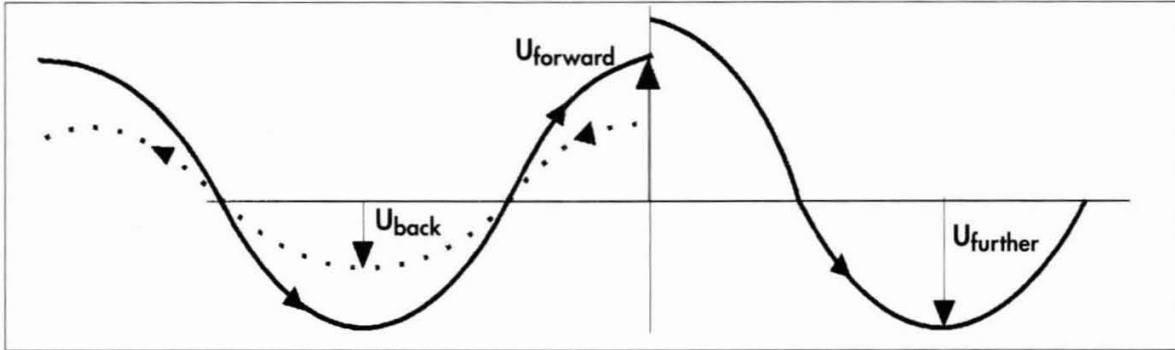
Figure 23 Reflected waves
