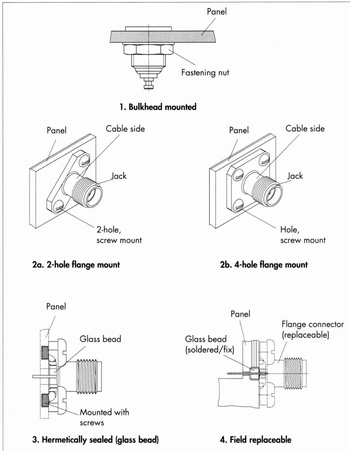
Figure 57 Panel-mounts
