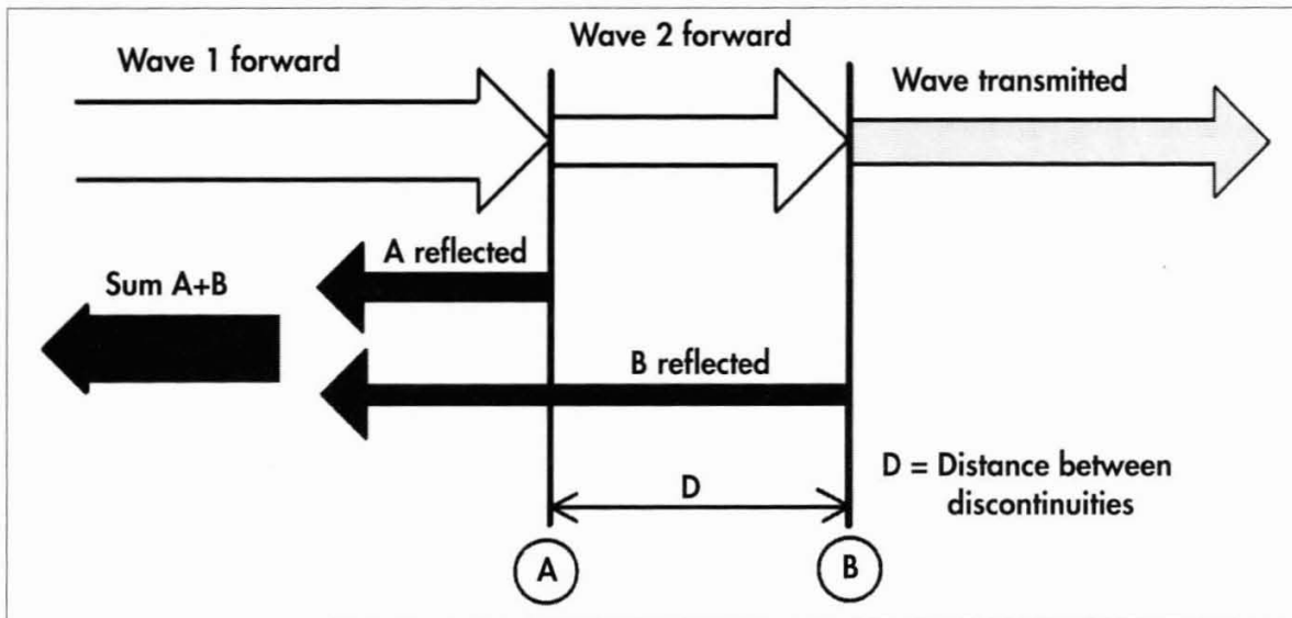
Figure 27 Reflections from several discontinuities
