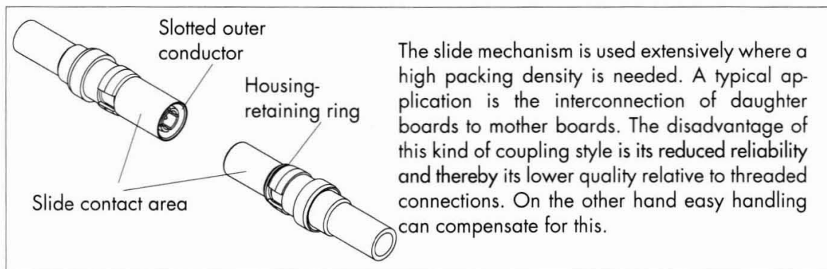
Figure 54 Slide-On coupling mechanism
