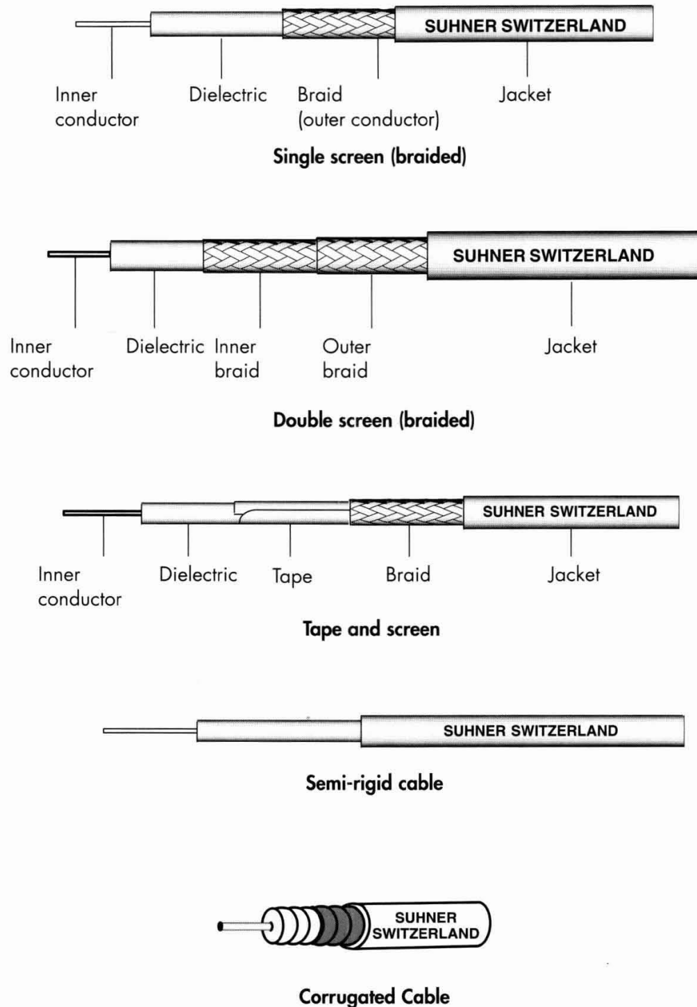
Figure 60 Cable designs
