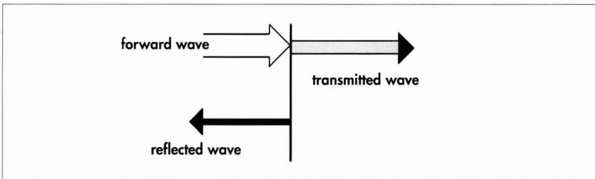
Figure 22 Waves reflected and transmitted at a discontinuity
