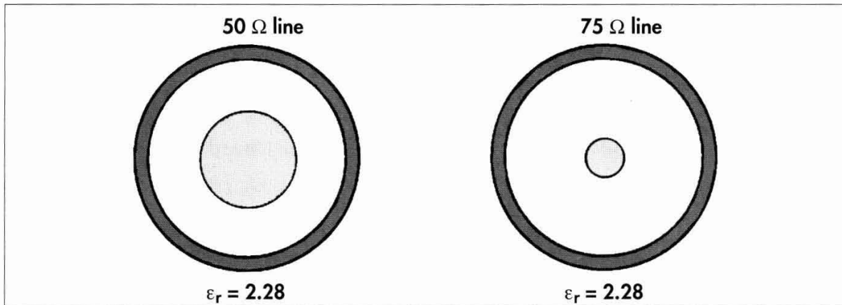
Figure 14 Different impedances caused by different insulator diameters
