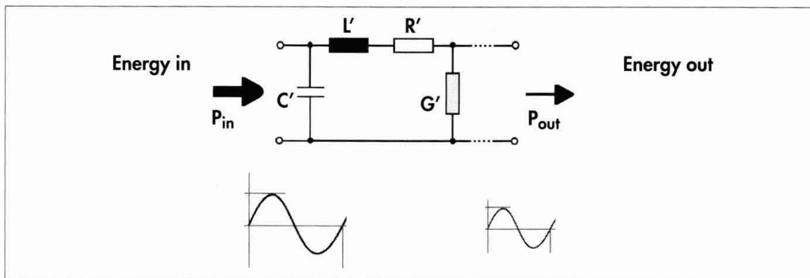
Figure 30 Attenuation loss (loss of energy) through the cable
