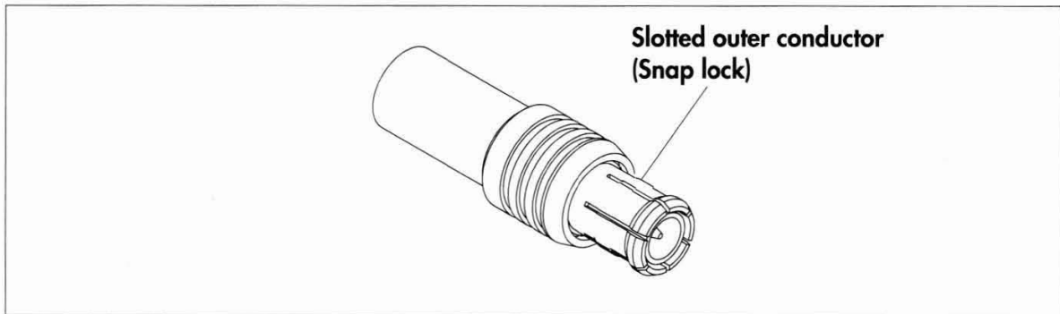
Figure 62 MCX plug connector (male)
