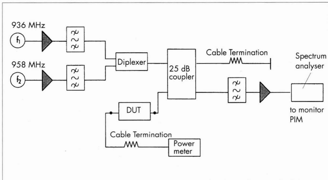
Figure 91 Schematic diagram of PIM test set-up (GSM, 900 MHz system)
