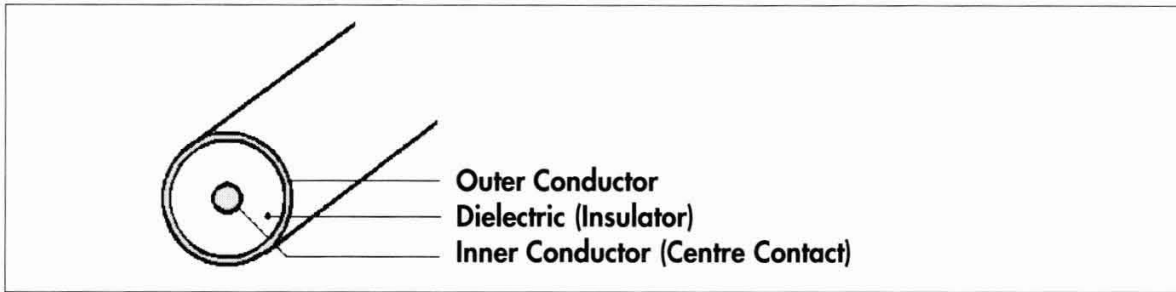
Figure 5 Construction of a RF line
