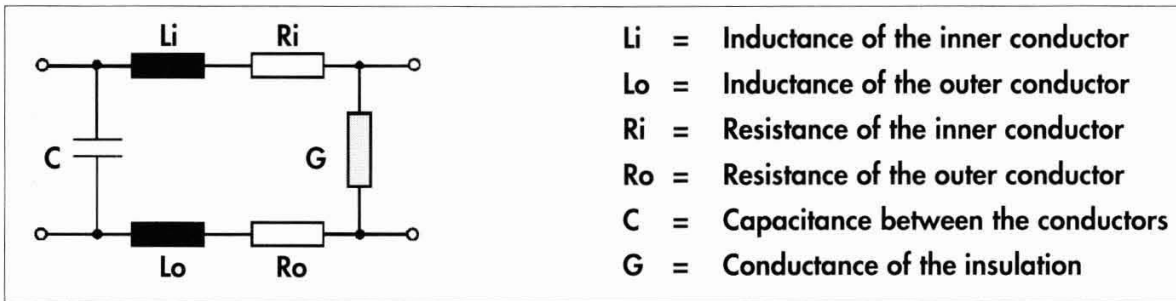
Figure 10 Equivalent circuit of RF line
