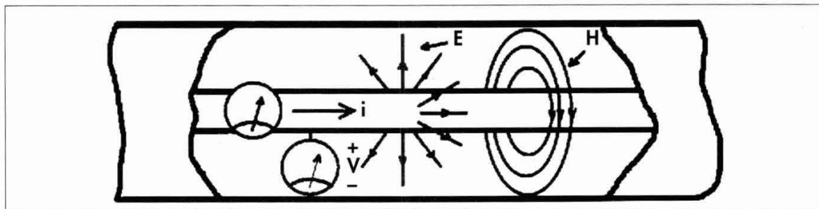
Figure 7 The electric and magnetic fields in a RF line
