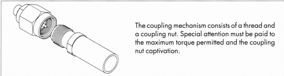
Figure 51 Threaded coupling mechanism
