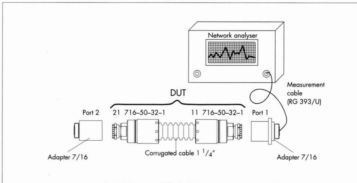
Figure 92 IM test set-up with 7/16 DUT
