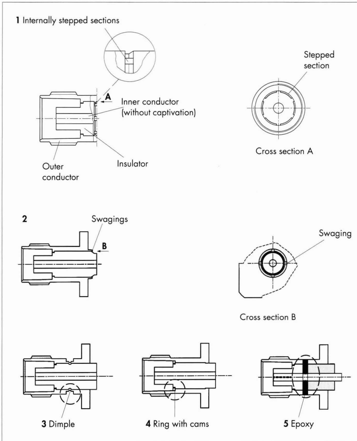
Figure 50 Various insulator captivation techniques
