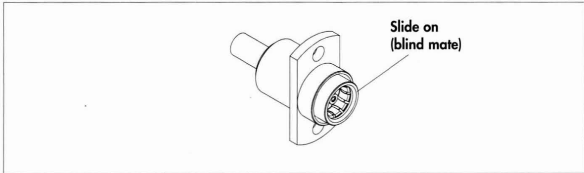
Figure 67 BMA plug connector
