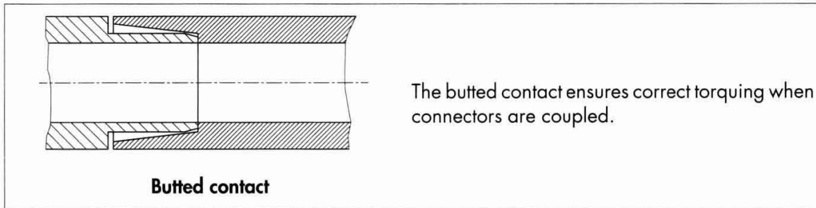
Figure 46 Butt faced outer conductor
