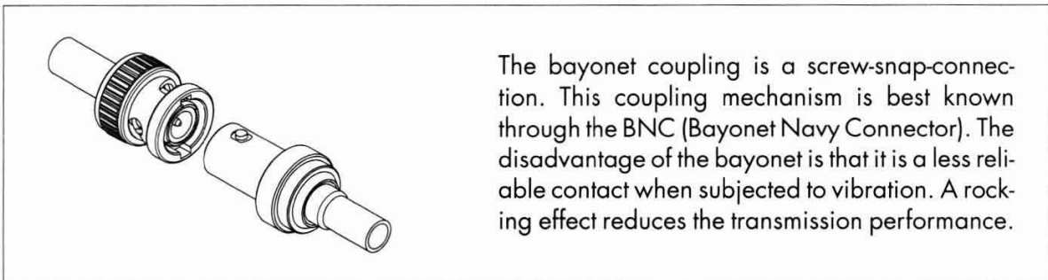
Figure 52 Bayonet coupling mechanism
