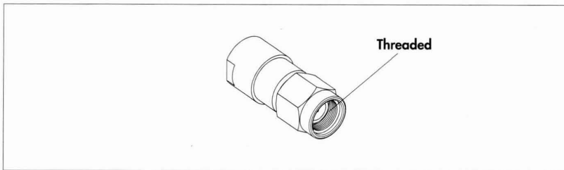
Figure 79 PC3.5 plug connector
