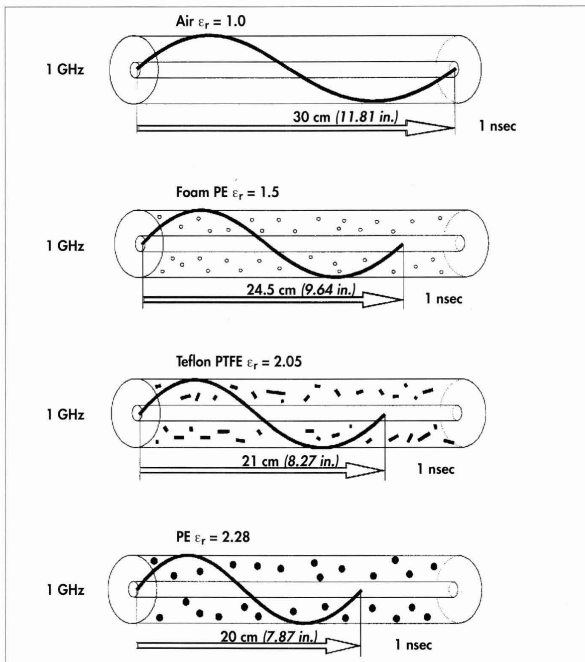
Figure 16 Wave propagation in various materials
