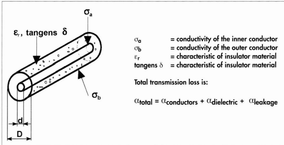
Figure 31 Attenuation loss components
