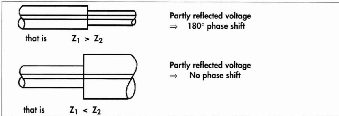
Figure 21 Phase shift as consequence of discontinuities
