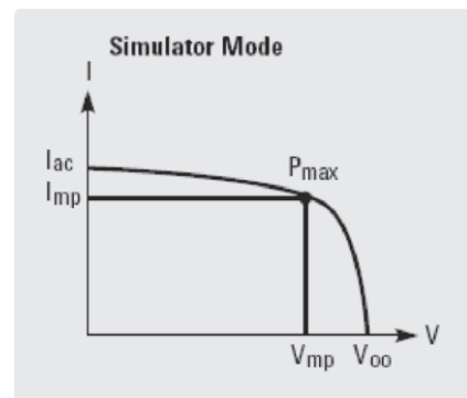
Figure 1: Power supply output characteristic in Simulator mode
