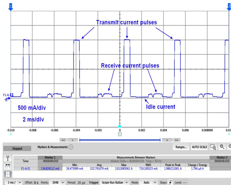
Figure1: GPRS smart phone active mode current drain waveform details.
