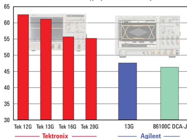
Total Jitter (ps) PRBS7 8 Gbps
