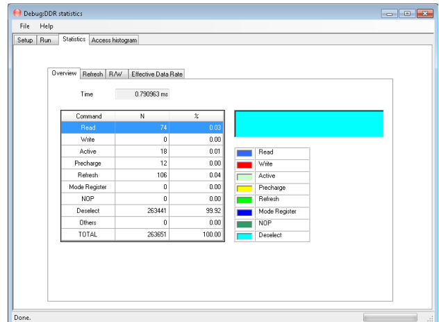
Performance test analysis of DDR3 Addr/Cmd line saved trace
