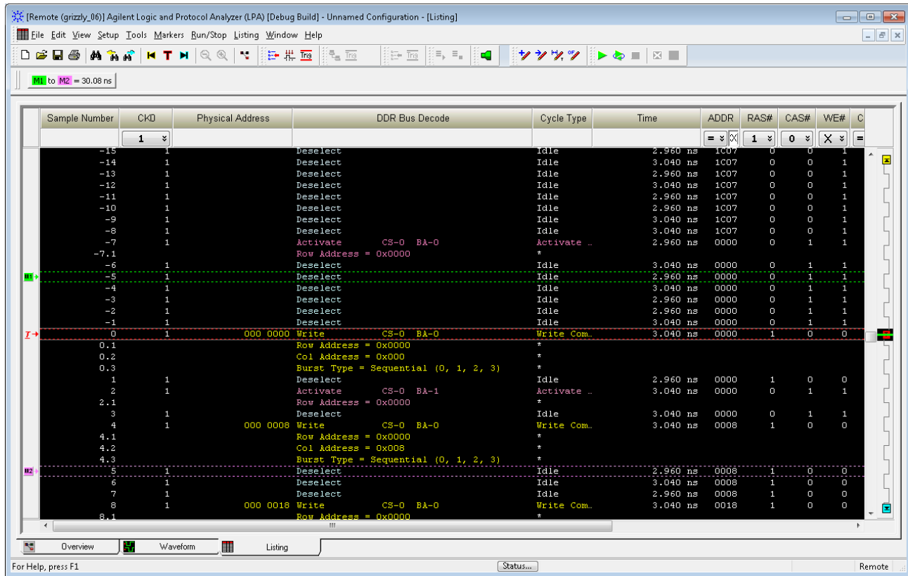
16850 Series capture and decode of DDR3 Addr/Cmd lines
