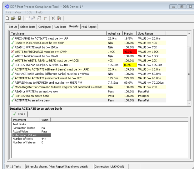
Compliance test analysis of DDR3 Addr/Cmd line saved trace
