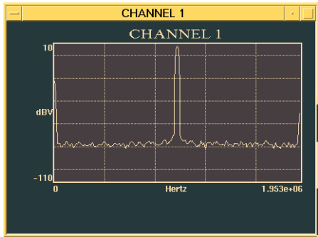
Magnitude-Squared spectrum from data acquired from the HP E1430 input module.
