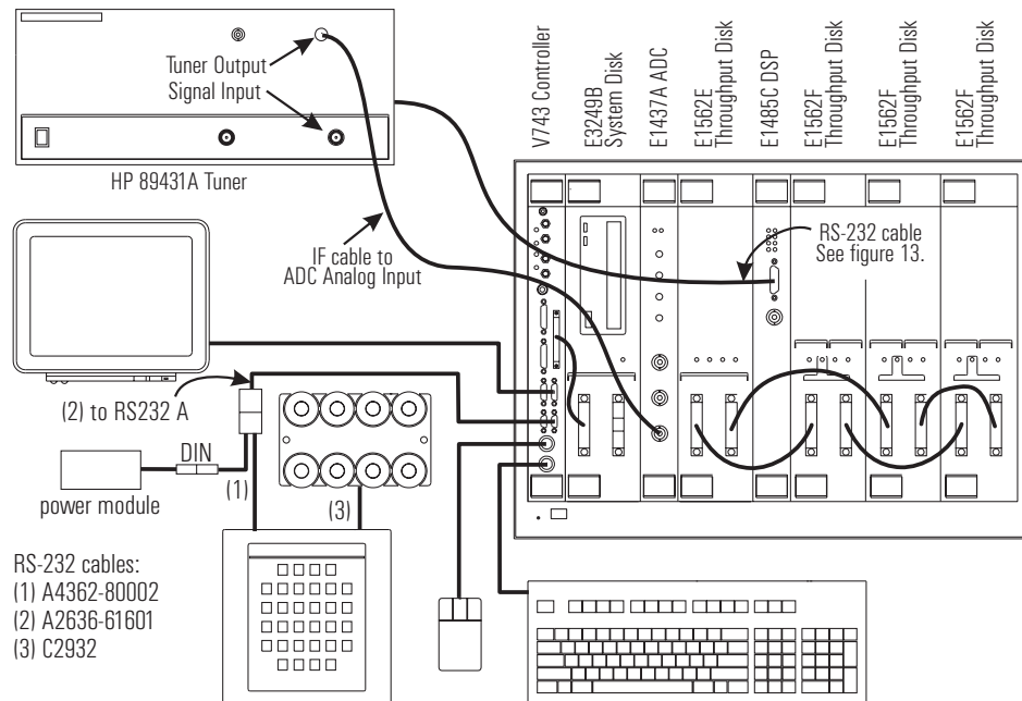
Figure 2. HP 3587S System Hardware Configuration incl. optional 2.65 GHz tuner & option ATR with 4 E1562 throughput disk modules
