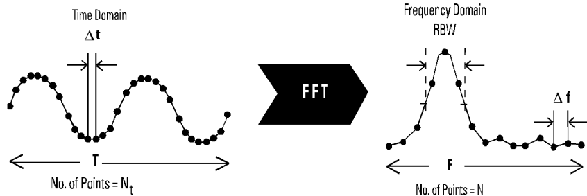
Figure 1. Description of FFT terms
