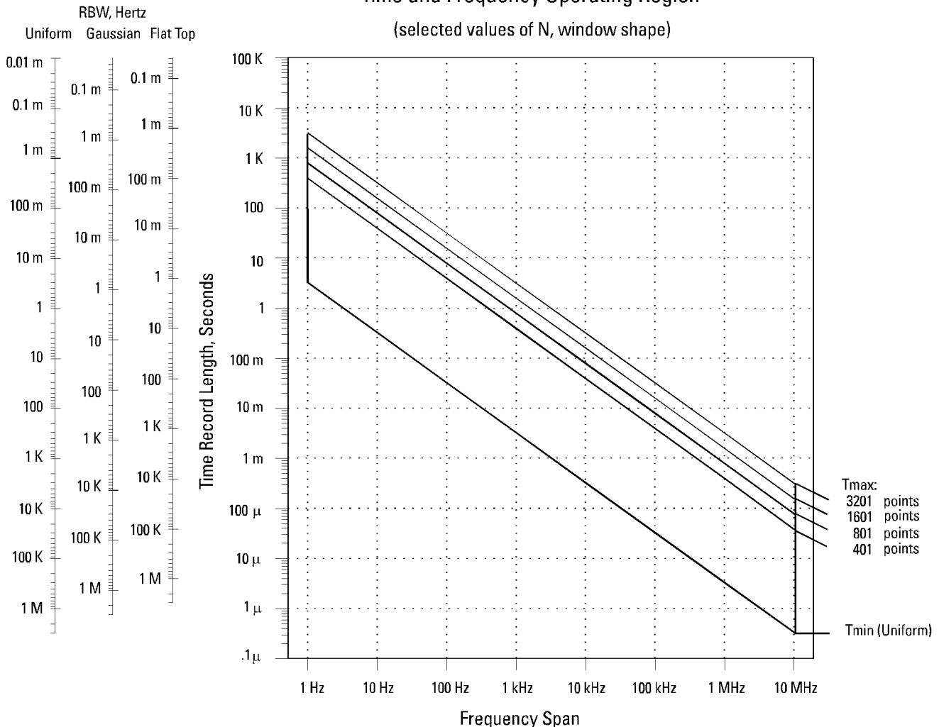
Figure 9. HP 89400 Series Vector Signal Analyzers Time and Frequency Operating Region
