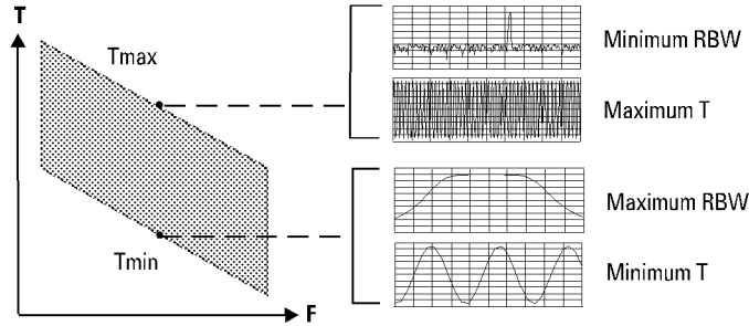
Figure 7. Time and frequency resolution tradeoffs within the HP 89400 operating region
