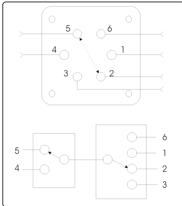
Figure 3. Matrix switch configured for 2x4 blocking application (RF path 5 to 2 shown)
