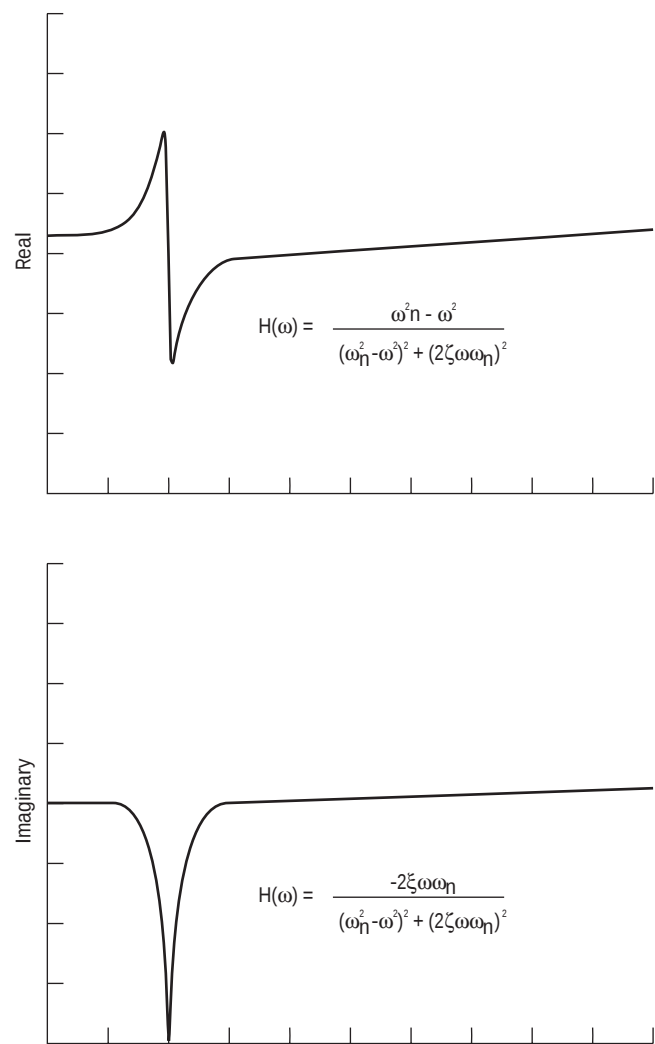
Figure 1.7 Frequency response — rectangular coordinates
