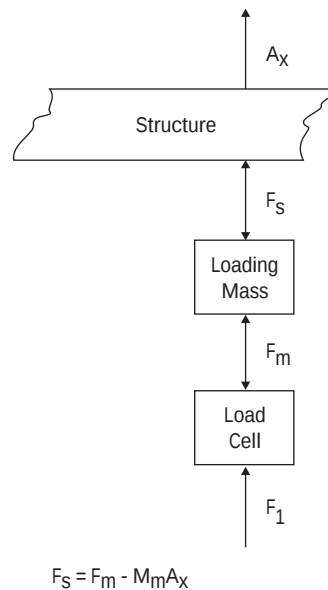
Figure 2.7 Mass loading from shaker setup
