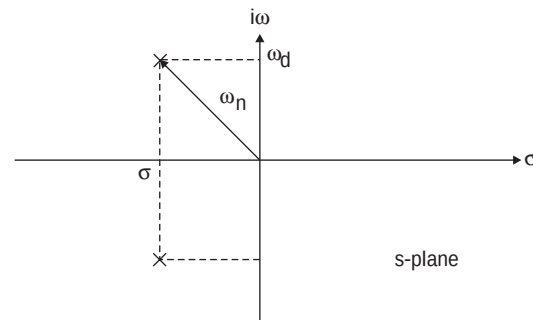
Figure 1.18 S-plane representation
