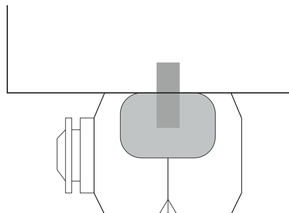
Figure 2.17 Stud mounted load cell
