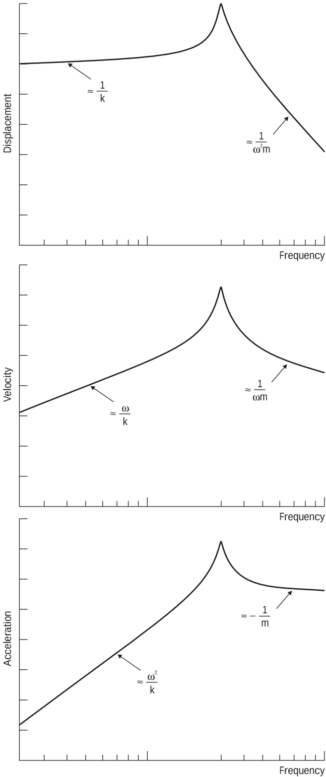
Figure 1.9 Different forms of frequency response
