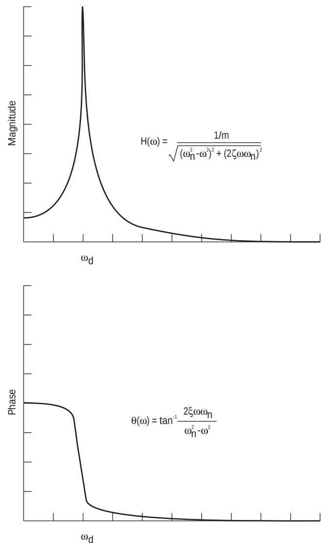
Figure 1.6 Frequency response — polar coordinates
