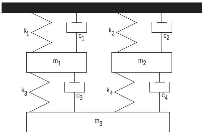
Figure 1.10 MDOF discrete parameter model
