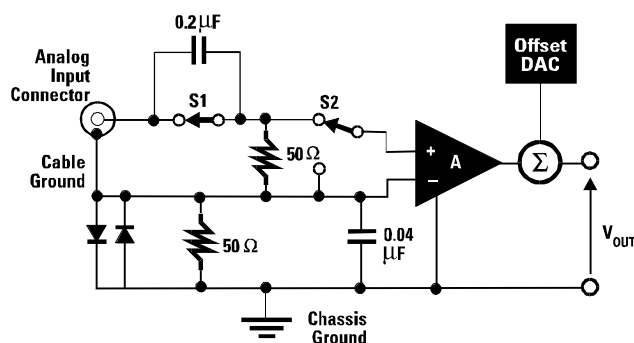
Fig. 3. Analog signal conditioning equivalent circuit.
