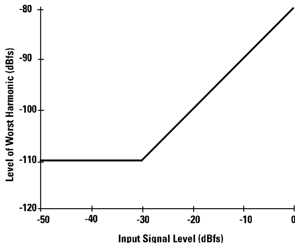
Fig. 4. Harmonic distortion as a function of input level
