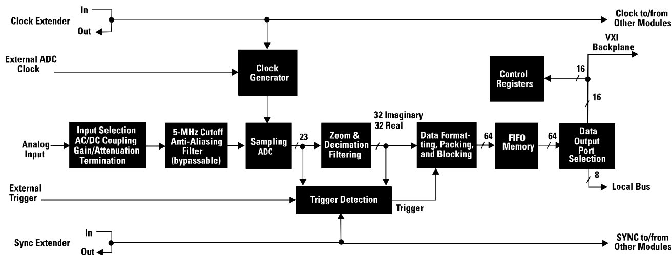
Fig. 2. Block diagram of the HP E1430A ADC module.
