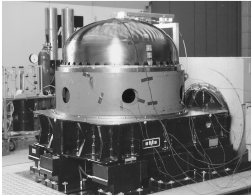
Figure 4: Testing a Propellant Tank
