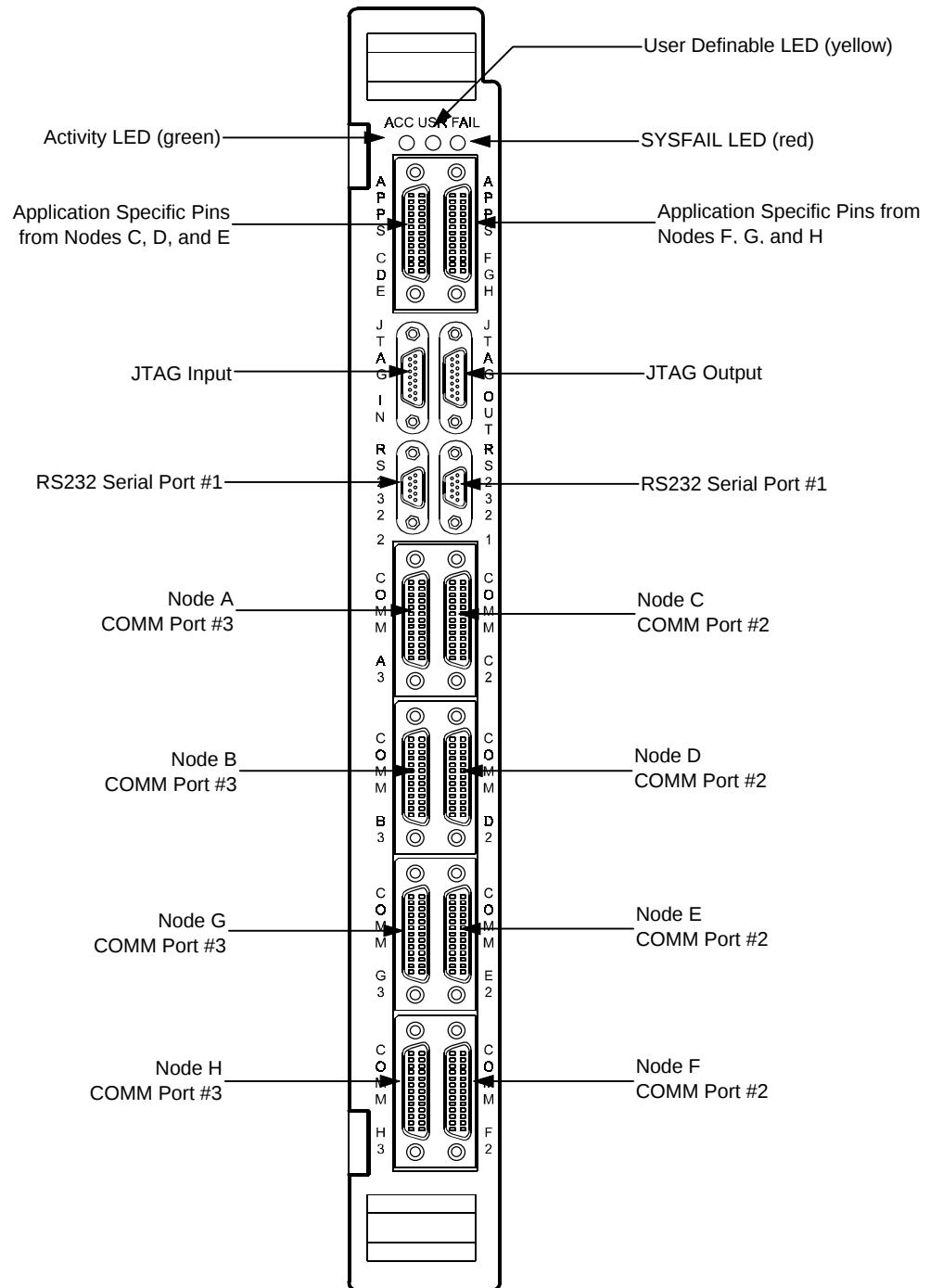
Figure 2 VX8 Front Panel
