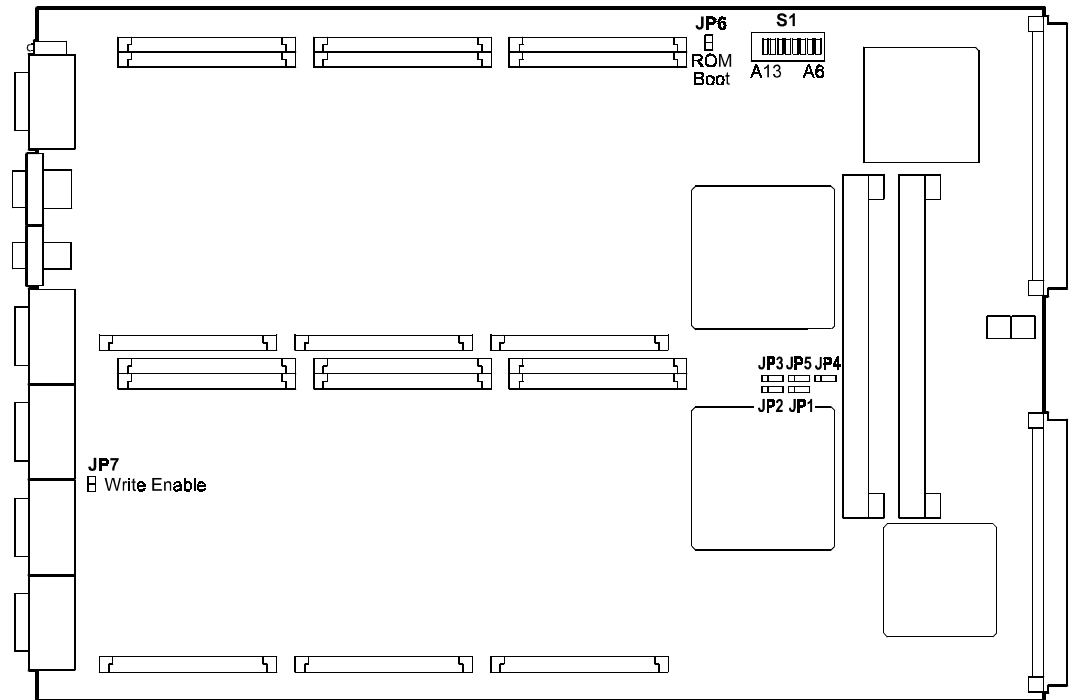
Figure 3 VX8 Jumper and Switch Locations
