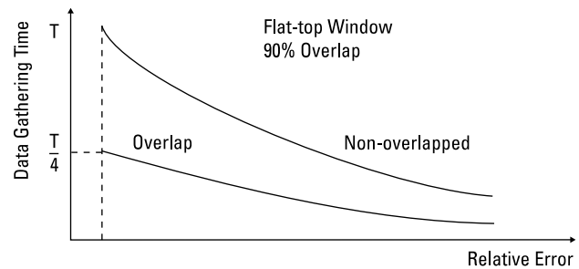
Figure 3.52 RMS averaging speed improve- ments with overlap processing.
