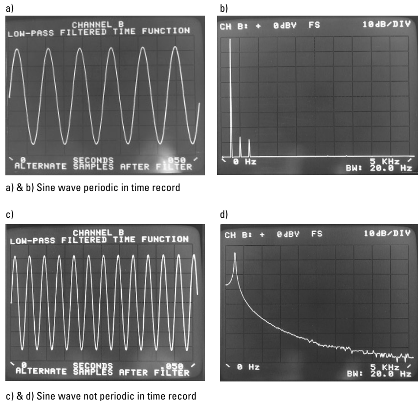
c) & d) Sine wave not periodic in time record
