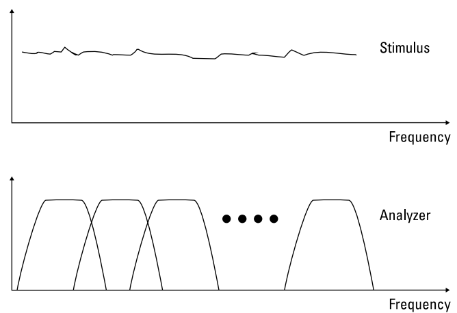
Figure 3.39 Random noise as a stimulus.
