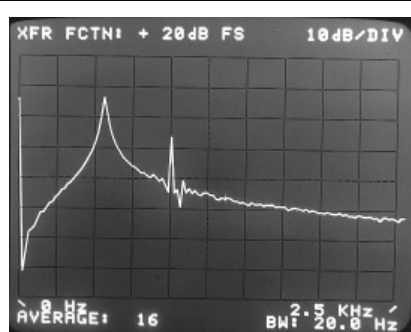
Figure 4.17 Magnitude and coherence of frequency response.
