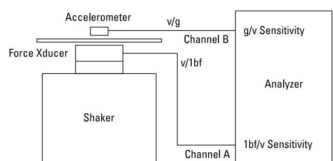
Figure 4.13 Engineering units set input sensitivities to properly scale results.
