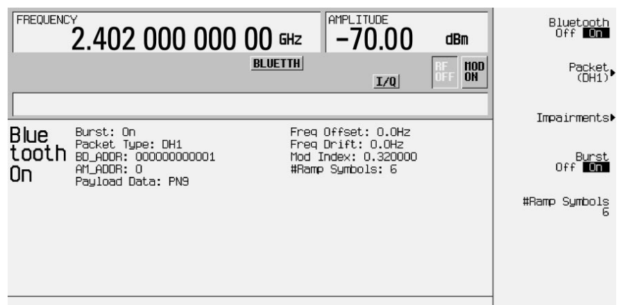
Figure 21. HP ESG-D series Option UND display of Bluetooth configuration menu
