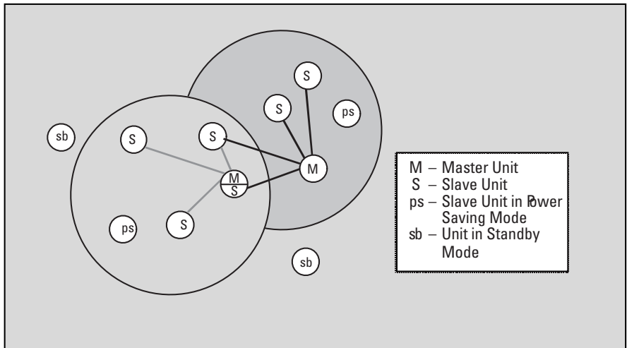
Figure 4. Network topology
