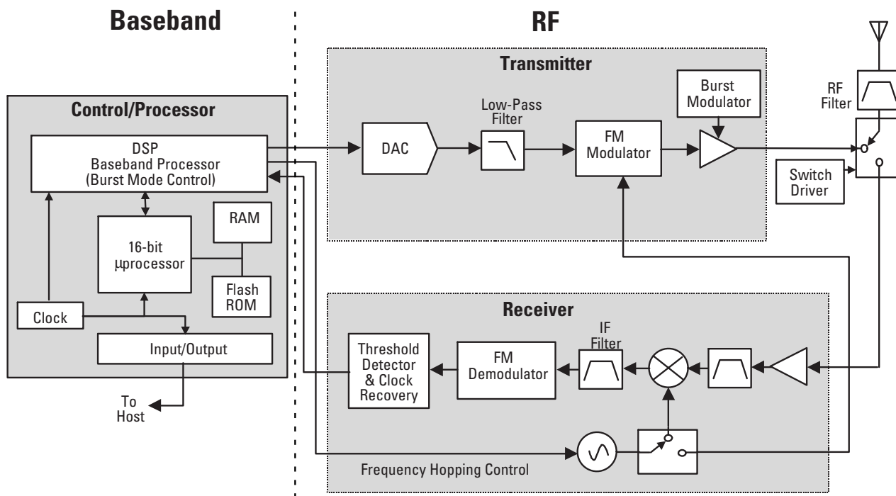
Figure 1. Block diagram of a Bluetooth system
