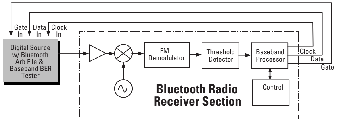
Figure 18. BER test setup using output of baseband processor
