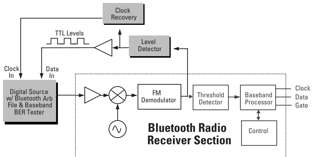
Figure 19. BER test setup using output of Bluetooth receiver's FM demodulator
