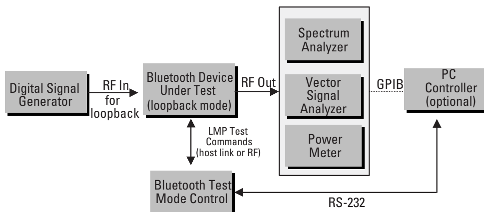
Figure 6. Transmitter measurement setup
