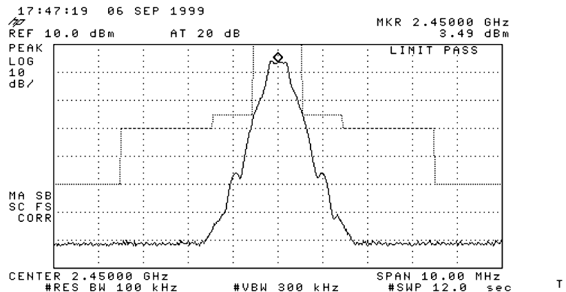
Figure 10. HP 8594E display of output spectrum measurement (CF=2.45 GHz, Span=10 MHz, RBW=100 kHz, VBW=300 kHz, Sweep Time=12 s, Detector Sample Mode, Trace Max Hold, Limit Line Mask.)
