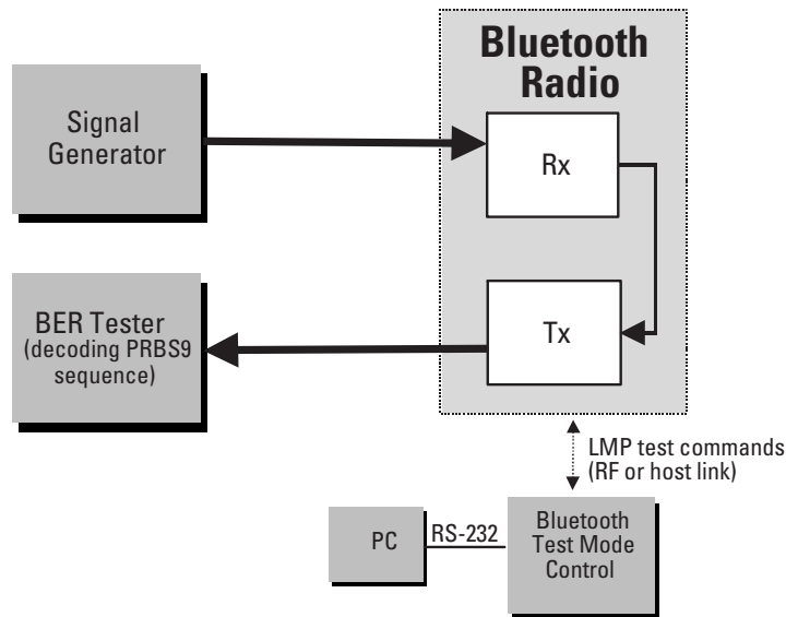
Figure 20. BER test setup using BER tester with Bluetooth device in test loopback mode
