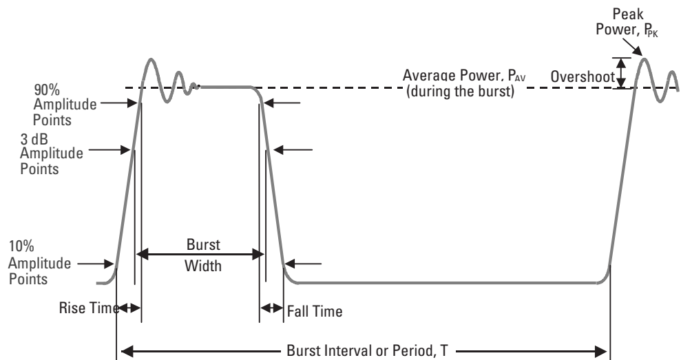
Figure 7. Time-domain power & timing analysis
