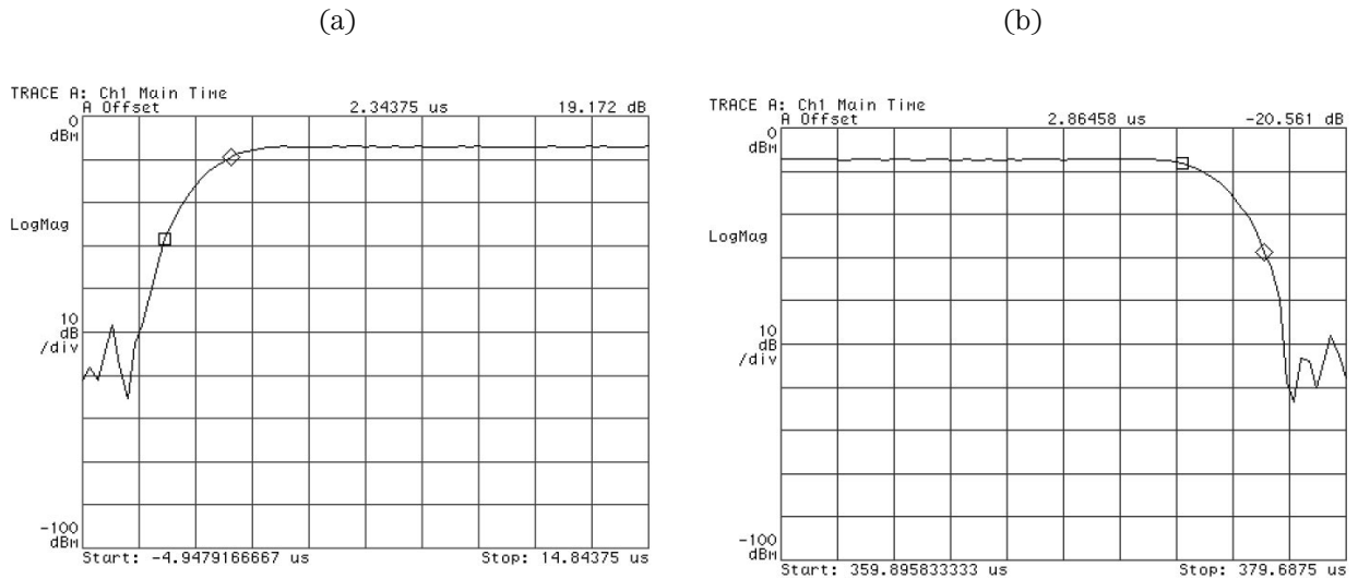
Figure 15. HP 89441A display showing burst (a) rise and (b) fall times (CF=2.45 GHz, Span=3 MHz, Vector mode, triggering on IF channel 1, main time ch1, magnitude log(dB), main length=20μs)
