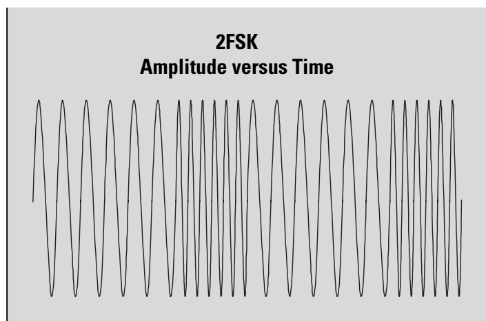
Figure 3. 2FSK modulation
