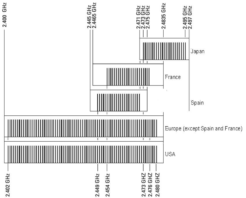
Figure 2. Bluetooth frequency channels
