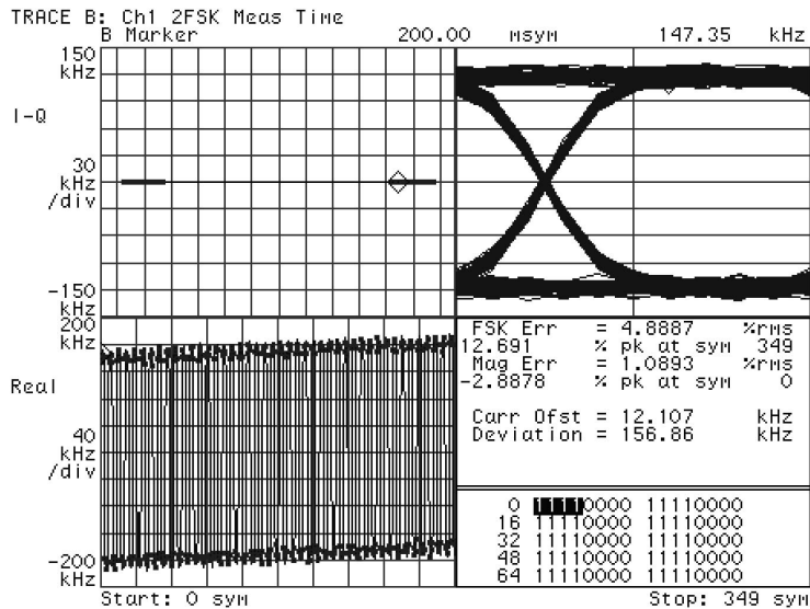
Figure 12. HP 8941A display of demodulation quality test
