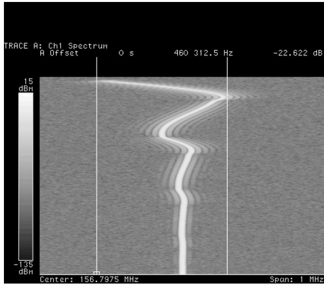
Figure 16. HP 89441A spectrogram display for PLL settling time
