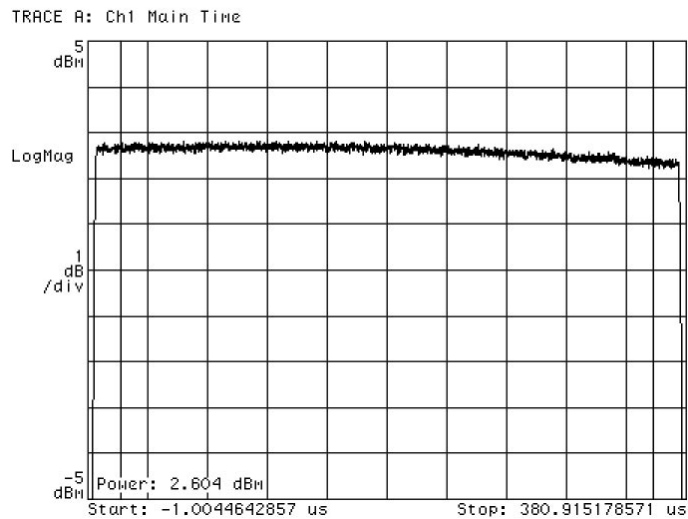
Figure 8. HP 89441A display of average and peak power measurement (CF=2.402 GHz, 1dB/div, sweep time=380 \mu s, triggering on IF ch 1, delay=1 \mu s)
