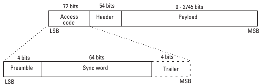
Figure 5. Bluetooth general packet format
