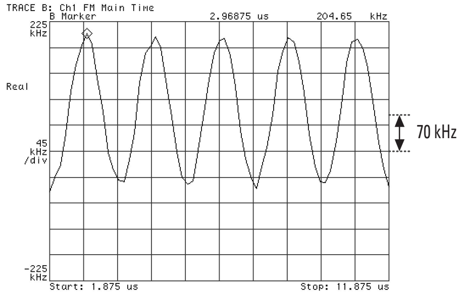
Figure 13. HP 89441A display of initial carrier frequency tolerance measurement with a 70 kHz frequency offset
