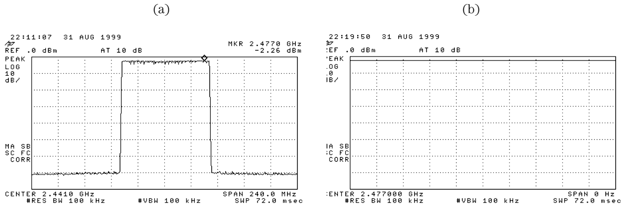
Figure 9. HP 8594E display of power density measurement
