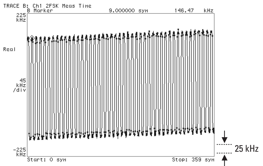
Figure 14. HP 8941A display of carrier frequency drift measurement
