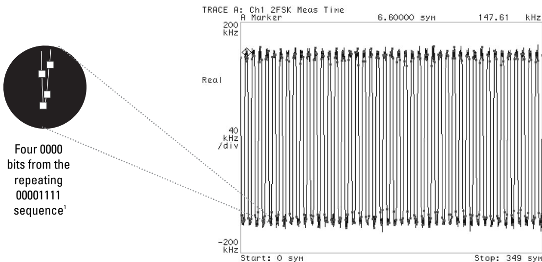
Figure 11. HP 8941A display showing modulation characteristics measurement. (CF=2.45 GHz, Demodulation mode, 2FSK, symbol rate=1MHz, triggering on IF channel 1, FSK measured time, part real (I), result length=350 symbols)
