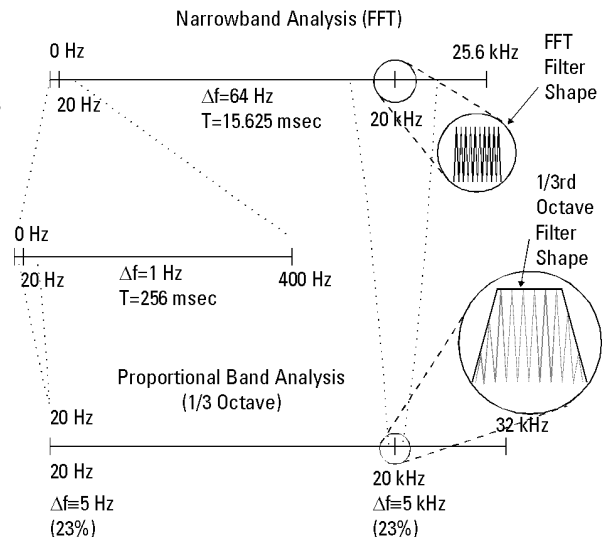
Figure 6.3-4 Synthesising 1/3 octave data from FFT requires multiple FFT bands of analyses. The lower frequencies of the 1/3 octave have resolution requirements of \Delta f = 5\text{ Hz} while the high frequencies require \Delta f = 5\text{ kHz} .
