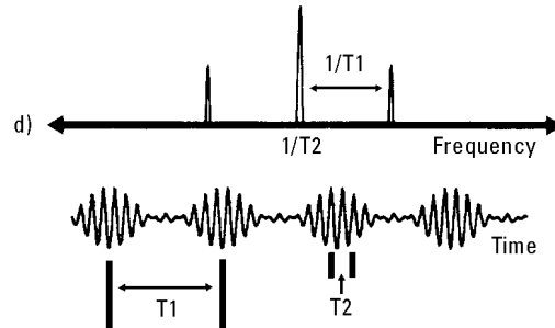
Figure 3.2-6 Examples of frequency spectra common in machinery vibration.
