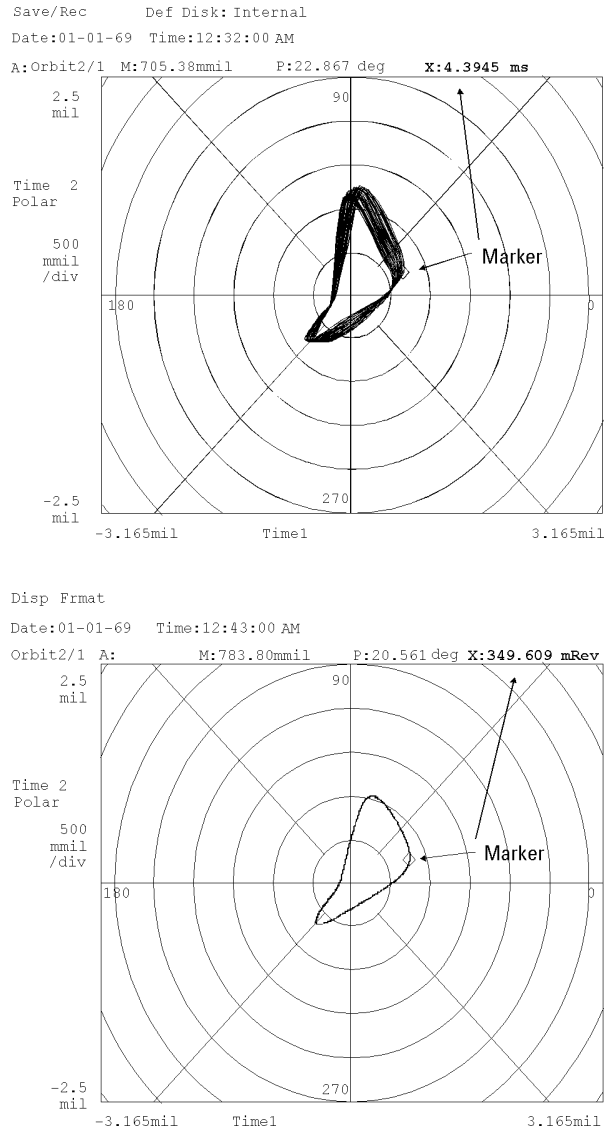
Figure 6.9-6 Orbit diagram using synchronous sampling will accurately represent the angular position (note the marker read out).
