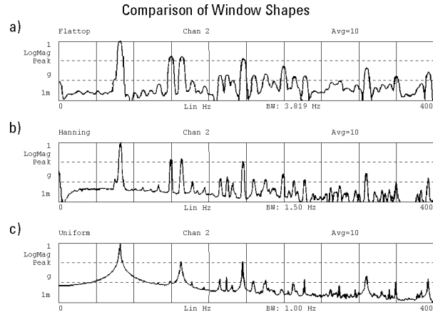
Figure 6.3-3 A comparison of 3 common window types: a) flat top, b) Hanning and c) uniform.
