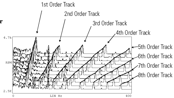
Figure 6.8-1 The order track is the locus of points of a particular order as a function of machine speed. Illustrated is the plot of this data super-imposed on a waterfall plot.
