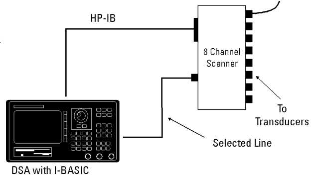
Figure 6.6-2 HP-IB system for scanning a number of transducers. Such a system can be configured to take appropriate action (e.g. sound an alarm or remove power) when current vibration level exceeds pre-defined limits.
