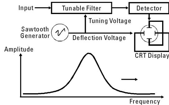
Figure 3.5-2 Swept filter analyzers provide better frequency resolution than parallel filter analyzers, but are too slow for machinery analysis.
