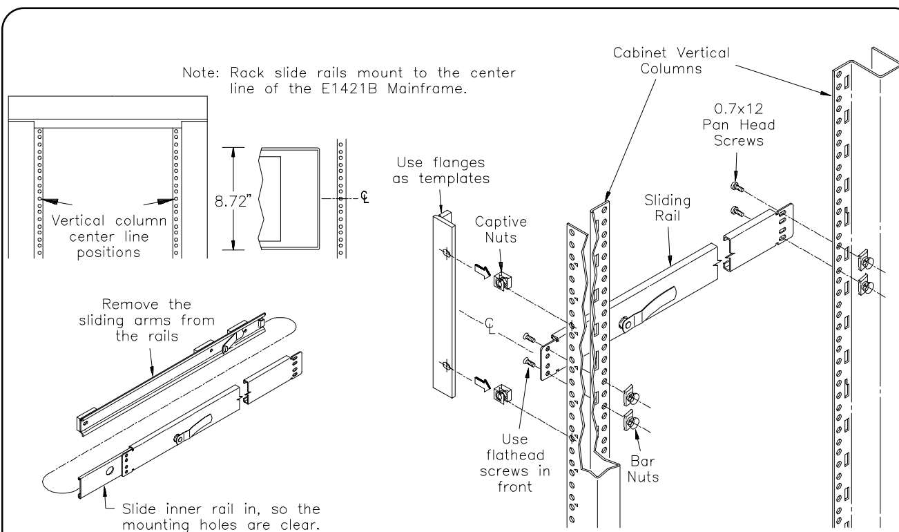
Figure 1-13. Mounting the Rack Slide Kit
