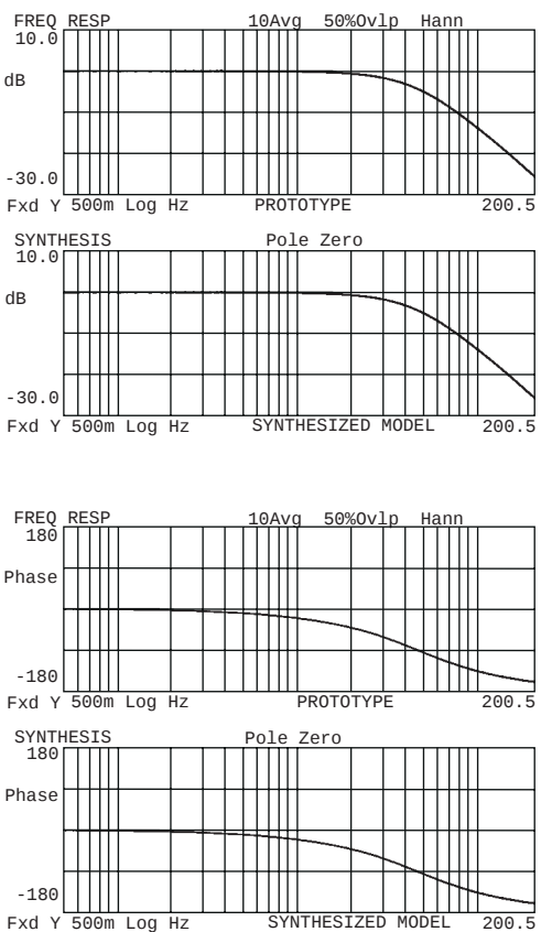
Figure 2-23: Measured frequency response of prototype (upper trace) compared to synthesized frequency response (lower trace).
