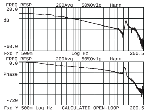
B. Calculated open-loop frequency response ( GH(j\omega) )
