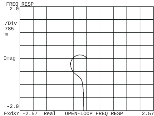
B. Nyquist plot
