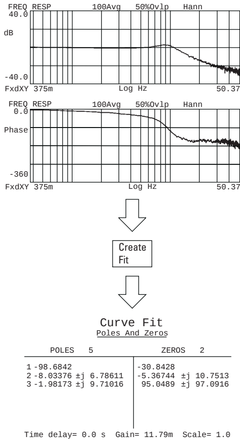
Figure 2-15: Using an MDOF curve fitter to estimate the pole/zero locations and gain from frequency response data.
