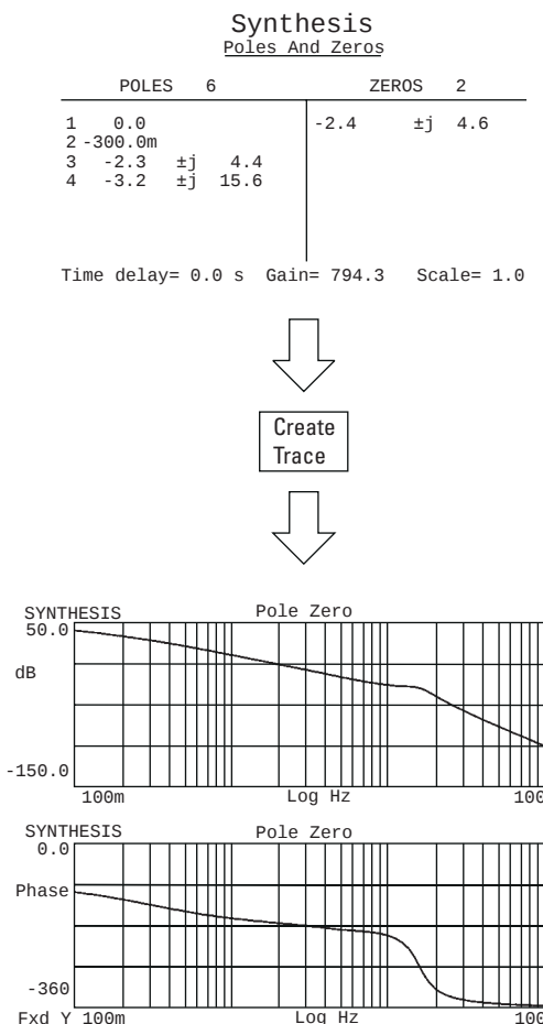
Figure 2-17: Synthesizing the frequency response of a control system using the DSA's frequency response synthesis function.
