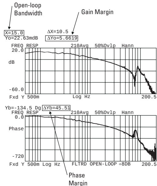
Figure 2-25: Measured open-loop frequency response with low-pass filter installed and gain increased by 8 dB.
