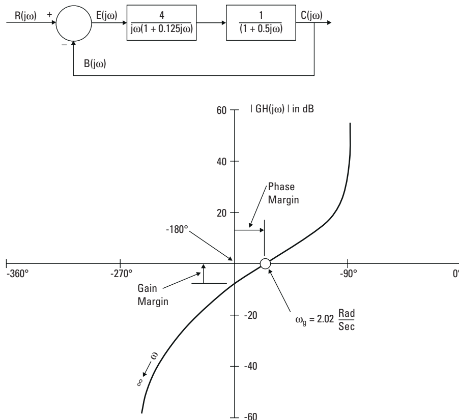
Figure 1-18: Nichols diagram (log magnitude versus angle diagram) for a typical open-loop transfer function.
