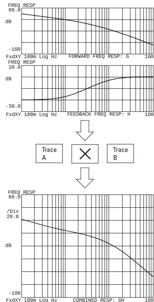
Figure 2-7: Using waveform math to combine frequency response data.
