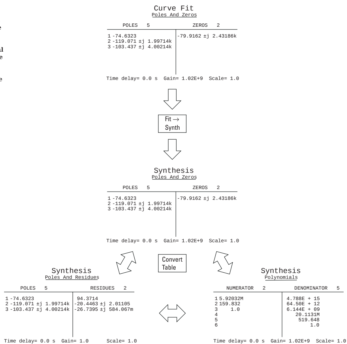
Figure 2-12: Converting pole/zero data from the curve fitter to pole/residue and polynomial formats via the frequency response synthesis table conversion function.
