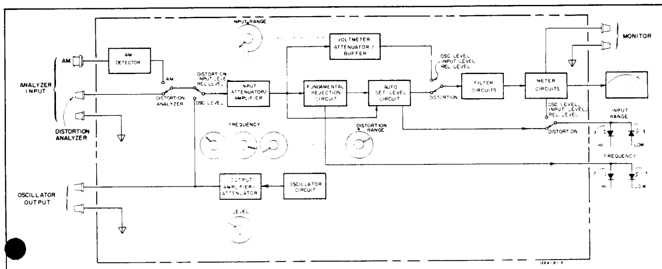
Figure 8-1. Model 339A Simplified Block Diagram.
