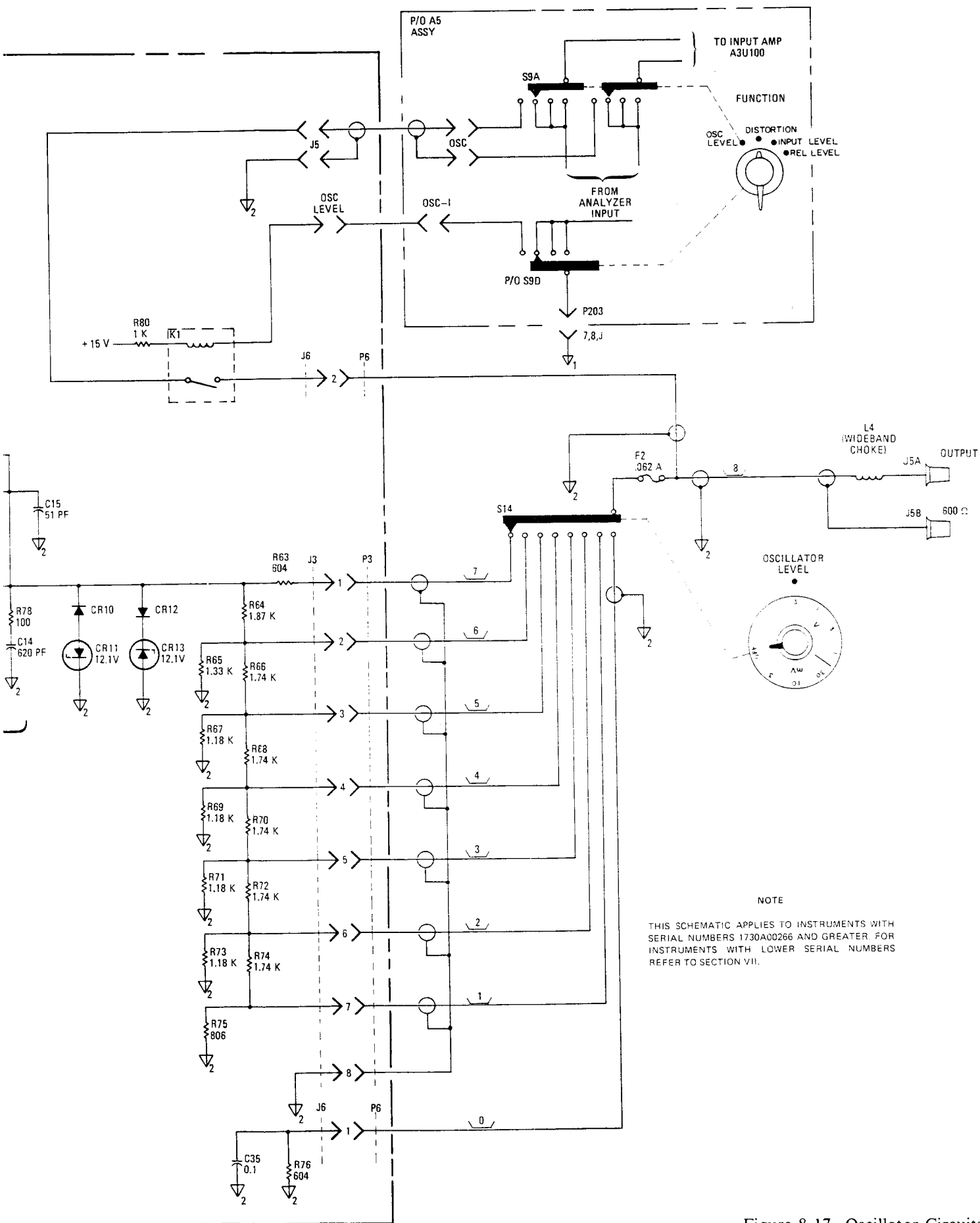
Figure 8-17. Oscillator Circuits. 8-21/8-22
