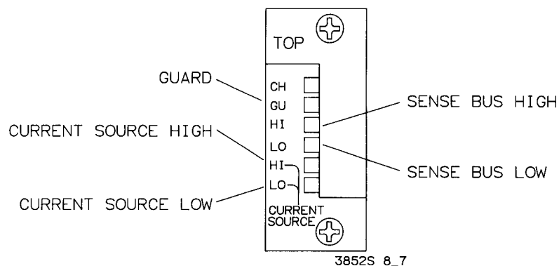
Figure 10-10 Analog Bus Connector
