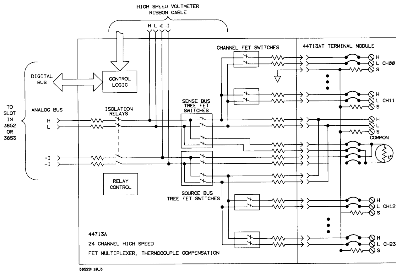
Figure 10-3 HP 44713A Simplified Schematic
