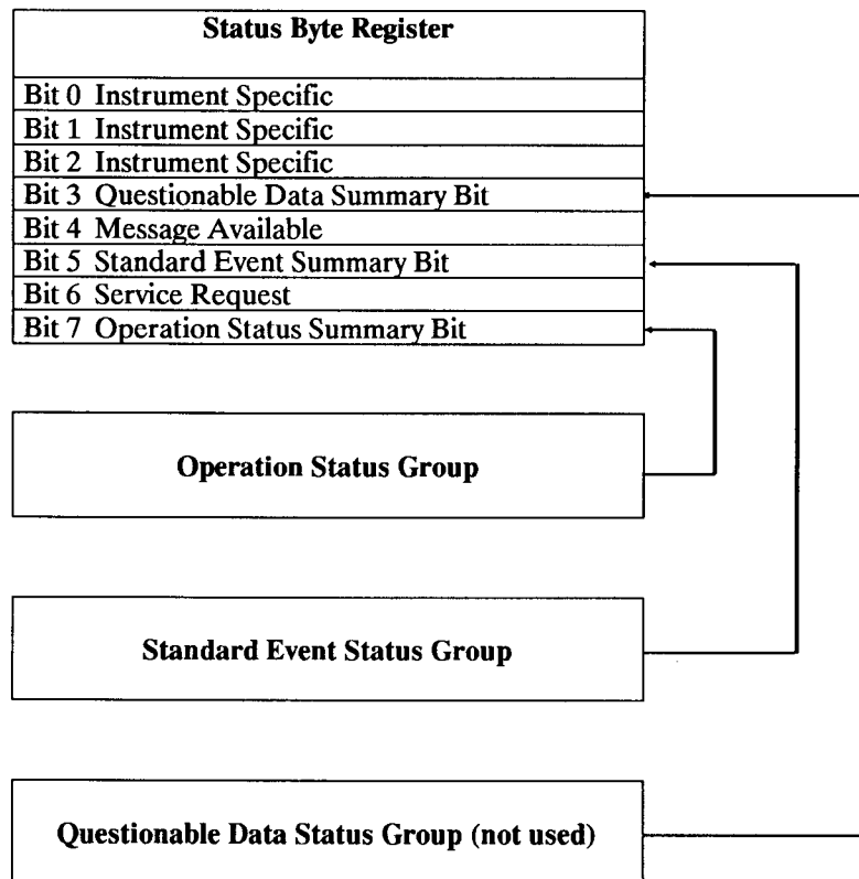
Figure 6-1. Status Structure
