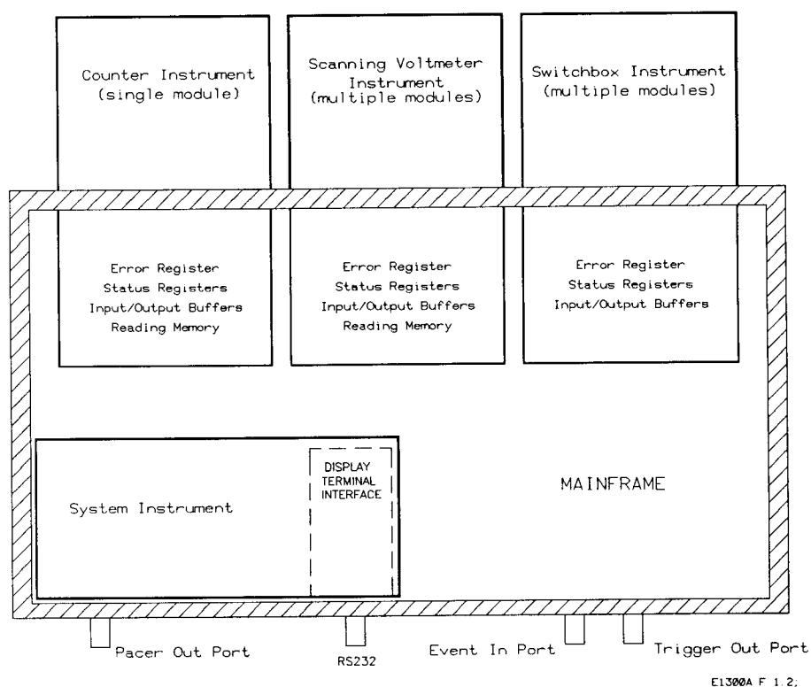
Figure 1-2. Instrument Concept
