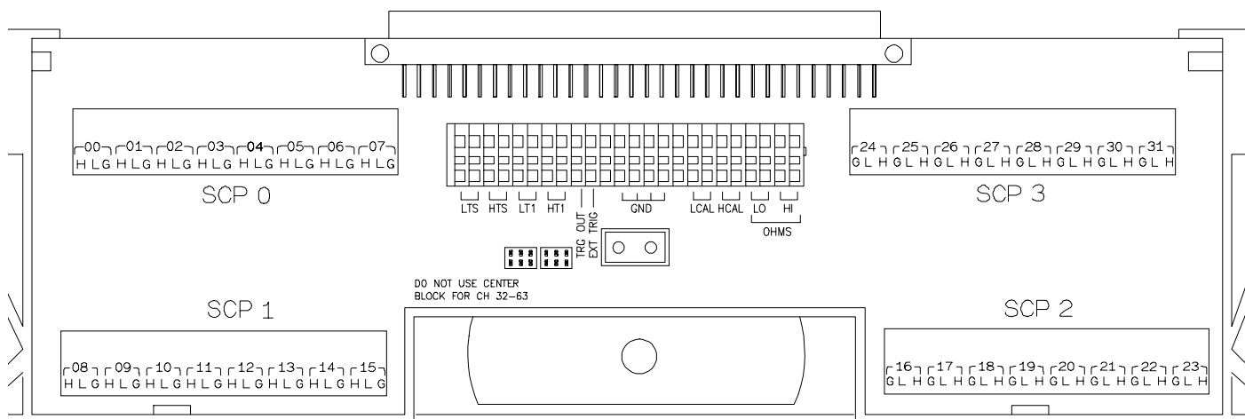
Figure 3 HP E1513 B-size Terminal Module Connections (Ch 00-31)
