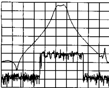
Figure 1. The HP 8751A gives you fast list sweeps with 130 dB dynamic range.
