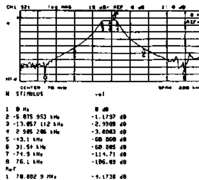
Figure 4. Key parameters are easy to measure and document with the marker page function.
