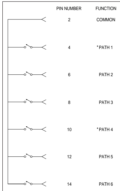
Figure 6. Pin function diagram
