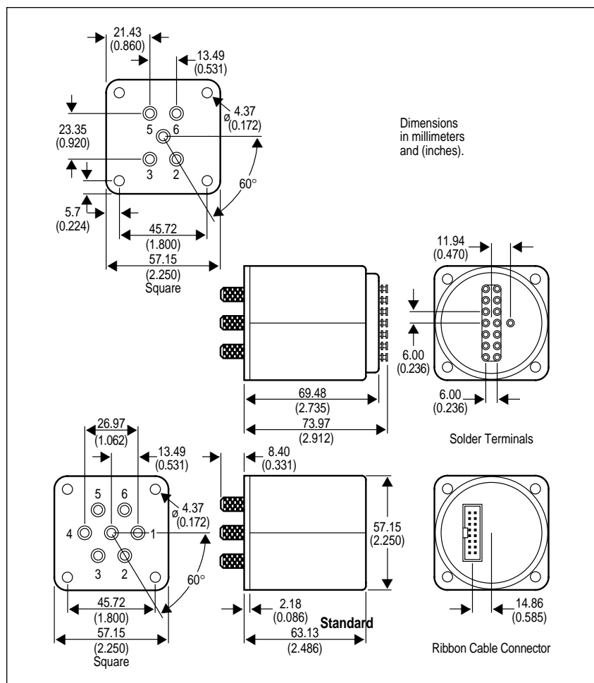
Figure 9. Product outlines
