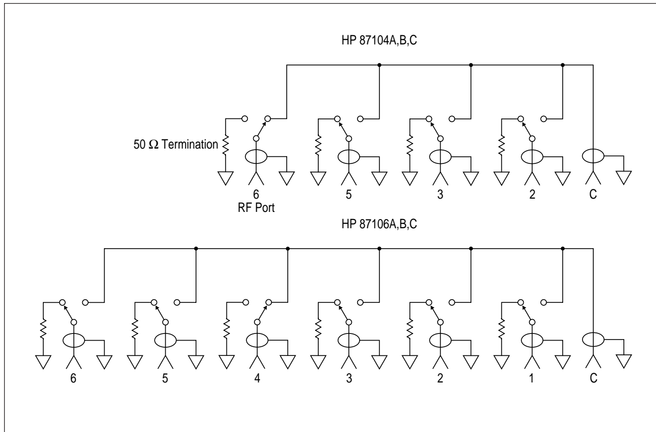
Figure 1. HP 87104A,B,C and 87106A,B,C simplified schematics.
