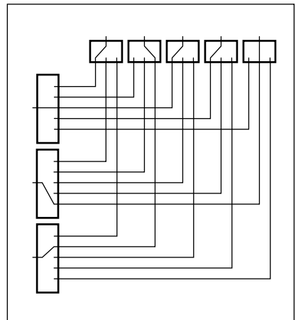
Figure 5. Full access matrix
