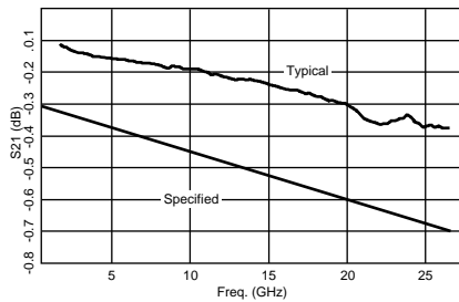
Figure 7. Insertion loss
