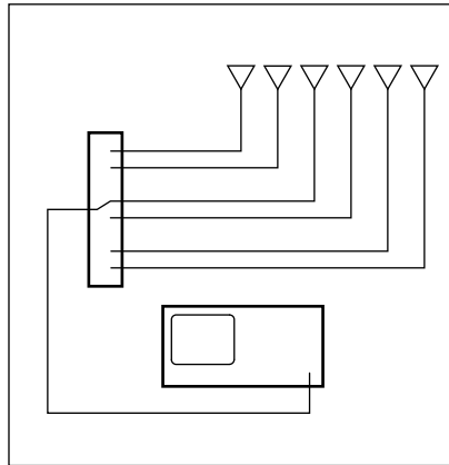
Figure 3. Multiport matrix
