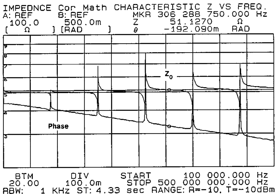
Figure 8. Characteristic Impedance Measurement Setup and Results
