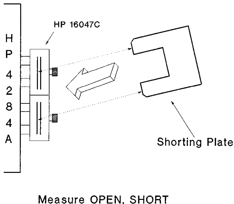
Figure 1. HP 4284A OPEN-SHORT Error Correction Measurement Setup
