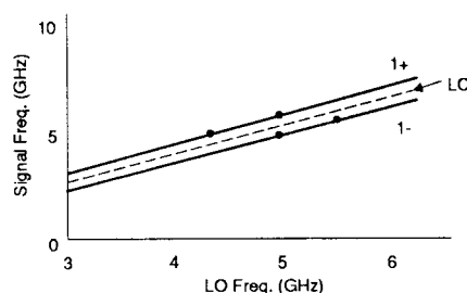
Figure 60. Tuning curves for fundamental mixing in the high-band, low-IF case
