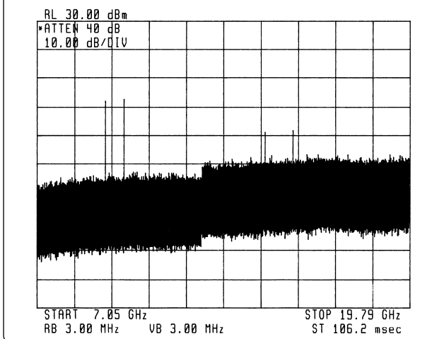
Figure 62. The number of responses is a function of signal frequency and analyzer span
