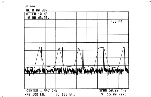
Figure 35. Pos peak display mode versus actual comb
