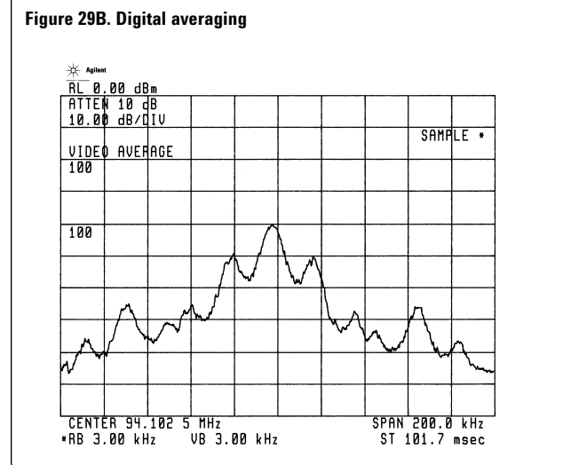
Figure 29. Video (analog) filtering and video (digital) averaging yield different results on an FM broadcast signal
