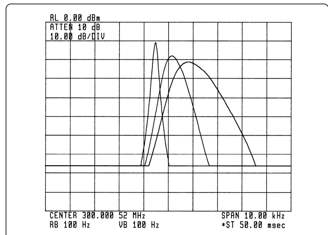
Figure 21. Sweeping an analyzer too fast causes a drop in displayed amplitude and a shift in indicated frequency
