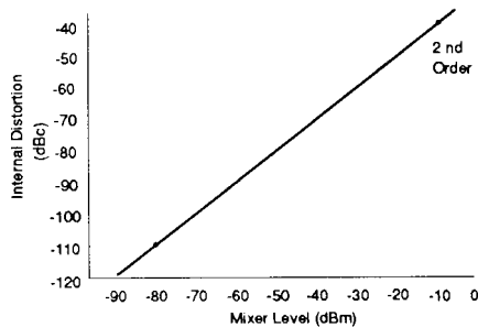
Figure 68. Extended second-order distortion graph
