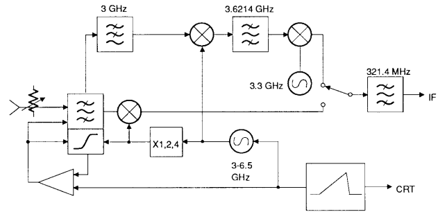
Figure 71. Front-end architecture of the Agilent 71210 with solid-state band switch, fundamental mixing to 22 GHz, and dynamic preselector peaking
