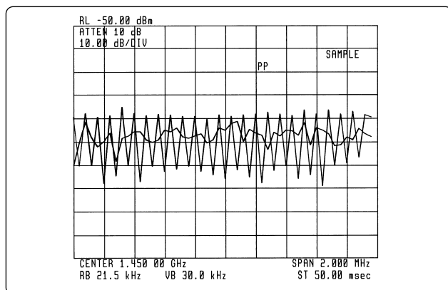
Figure 37. Comparison of Rosenfell and sample display modes
