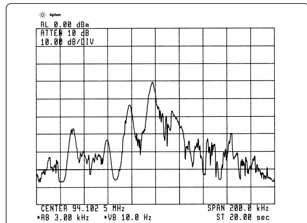
Figure 29A. Analog filtering
