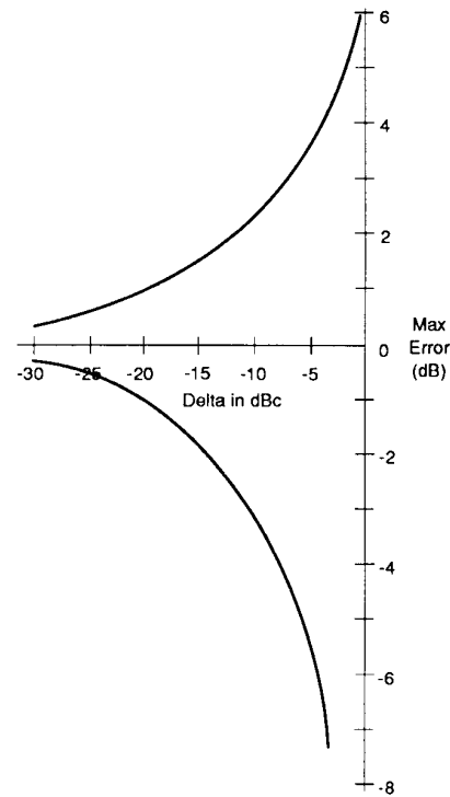
Figure 54. Uncertainty versus difference in amplitude between two sinusoids at the same frequency
