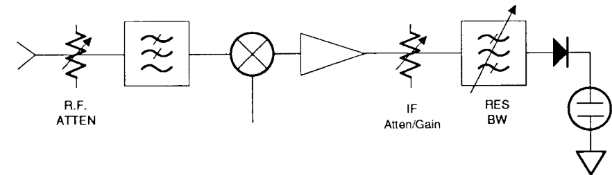
Figure 40. Controls that affect amplitude accuracy
