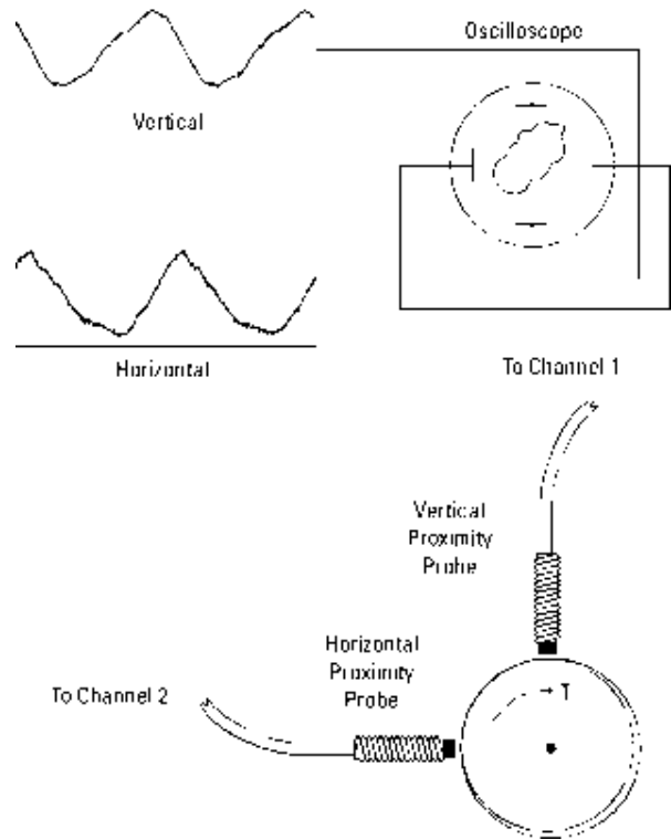
Figure 6.9-4 Measurement setup for orbit measurements using orthogonal proximity probe and a 2 channel DSA.
