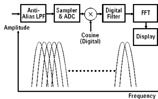
Figure 3.5-3 DSAs digitally simulate hundreds of parallel filters, providing both high speed and excellent frequency resolution. DSAs also provide time and phase displays not available on the other frequency domain analyzers.
