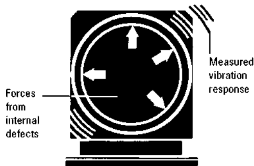
Figure 2.1-5 Vibration measured on a machine is the response to defect force, not the force itself.
