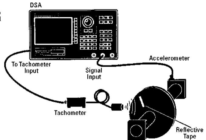
Figure 3.3-2 Set-up of DSA to produce spectral map.
