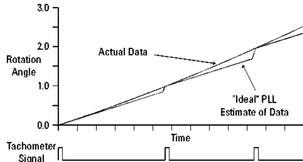
Figure A-4 Deviation of an "ideal" PLL's estimate of shaft angular position from actual shaft with constantly increasing RPM.
