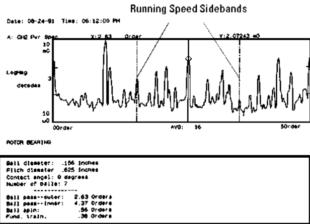
Figure 4.2-4 HP Instrument Basic print out of bearing data and characteristic frequencies with corresponding spectra. The result of a single defect on outer race is evident.
