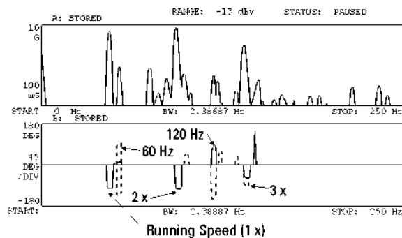
Figure 5.2-1 A sequence of vibration spectra with phase shows constant phase for imbalance (1 x and harmonics), and unstable phase for power-line components (60 Hz harmonics).
