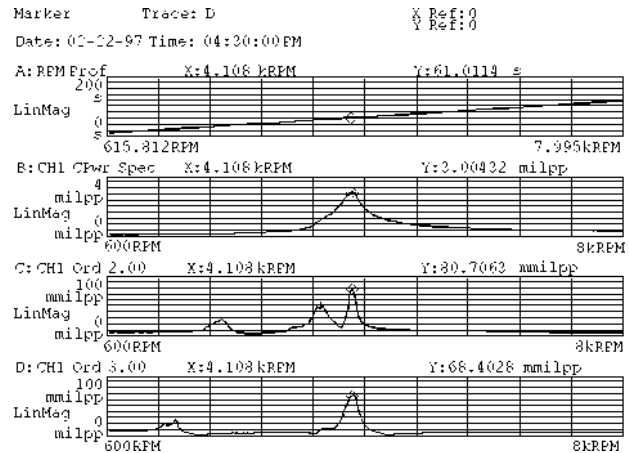
Figure 6.8-5 Runup depiction of the 2nd and 3rd orders as well as the overall level and the RPM profile.
