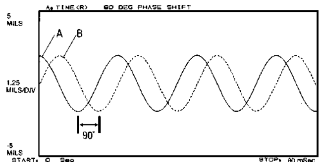
Figure 3.4-2 Two sine waves with a phase relationship of 90°.
