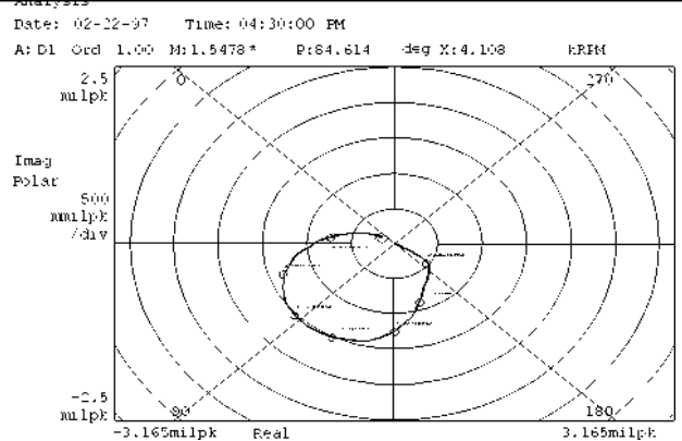
Figure 6.8-4(b) Polar plot of runup depicting the magnitude and phase plotted in a polar fashion. Note the rotation intended to compensate for positioning of the phase reference and the displacement transducer.
