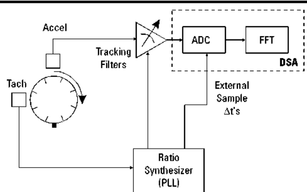
Figure A-1 Traditional external sampling method of order domain analysis.
