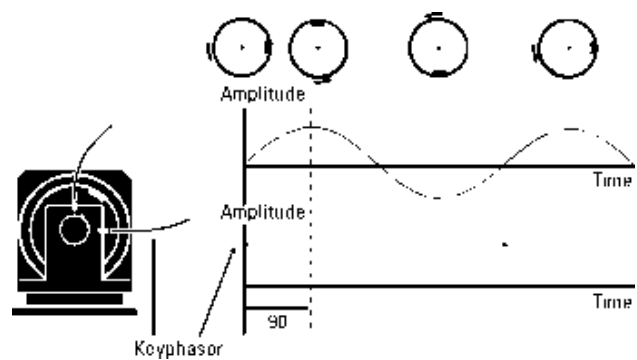
Figure 3.4-4 Since the heavy spot on the rotor passes the transducer 90° after the keyway passes the keyphasor, the imbalance signal lags the keyphasor pulse by 90°. The corresponding frequency domain phase spectrum is shown in Figure 3.4-3.
