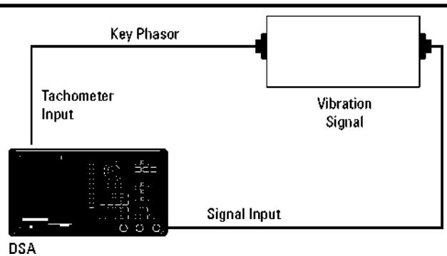
Figure 6.8-3 Instrumentation for synchronous sample control for DSA with digital synchronous resampling.
