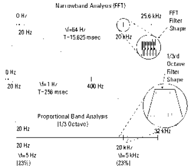
Figure 6.3-4 Synthesising 1/3 octave data from FFT requires multiple FFT bands of analyses. The lower frequencies of the 1/3 octave have resolution requirements of \Delta f 5Hz while the high frequencies require \Delta f 5kHz.
