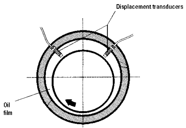
Figure 2.1-6 A relatively light shaft turning in fluid-film bearings transmits little vibration to the machine housing. Its vibration must be measured directly with a displacement transducer.
