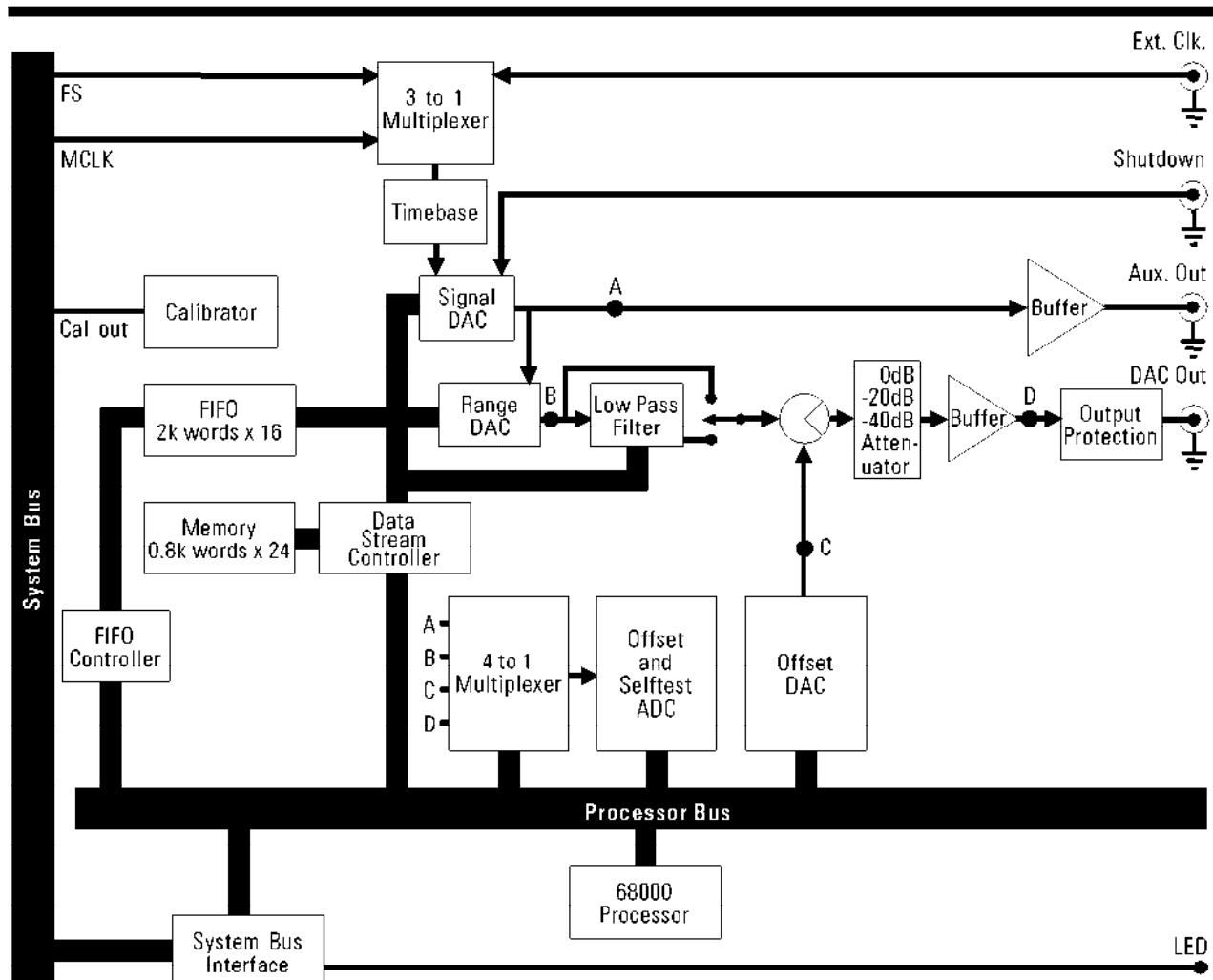
HP 35656B Block Diagram
