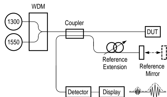
Precision lightwave reflectometer block diagram
