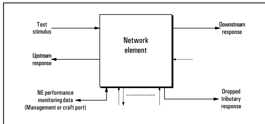
Figure 1. Connecting to network element under test
