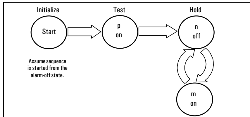
Figure 2. Testing alarm detection and de-activation thresholds
