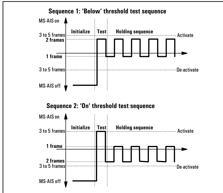
Figure 3. MS-AIS detection threshold test
