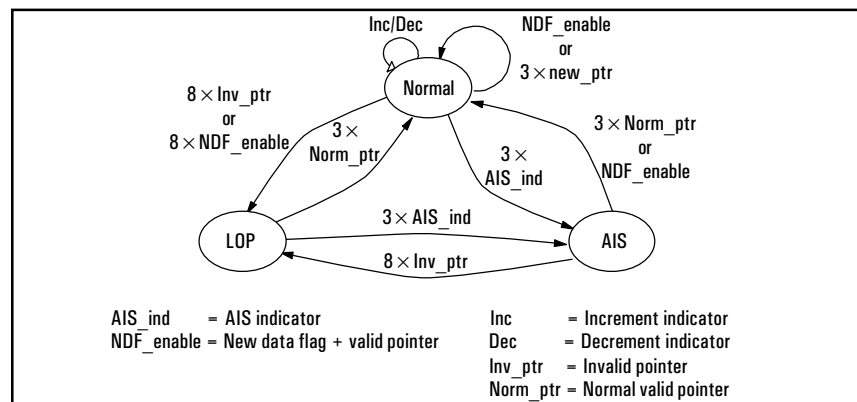
Figure 4. Pointer operation: ETSI TM-1015
