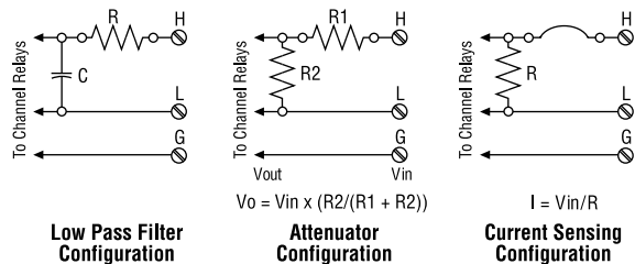
Signal conditioning components and current shunt for HP E1351A/52A
