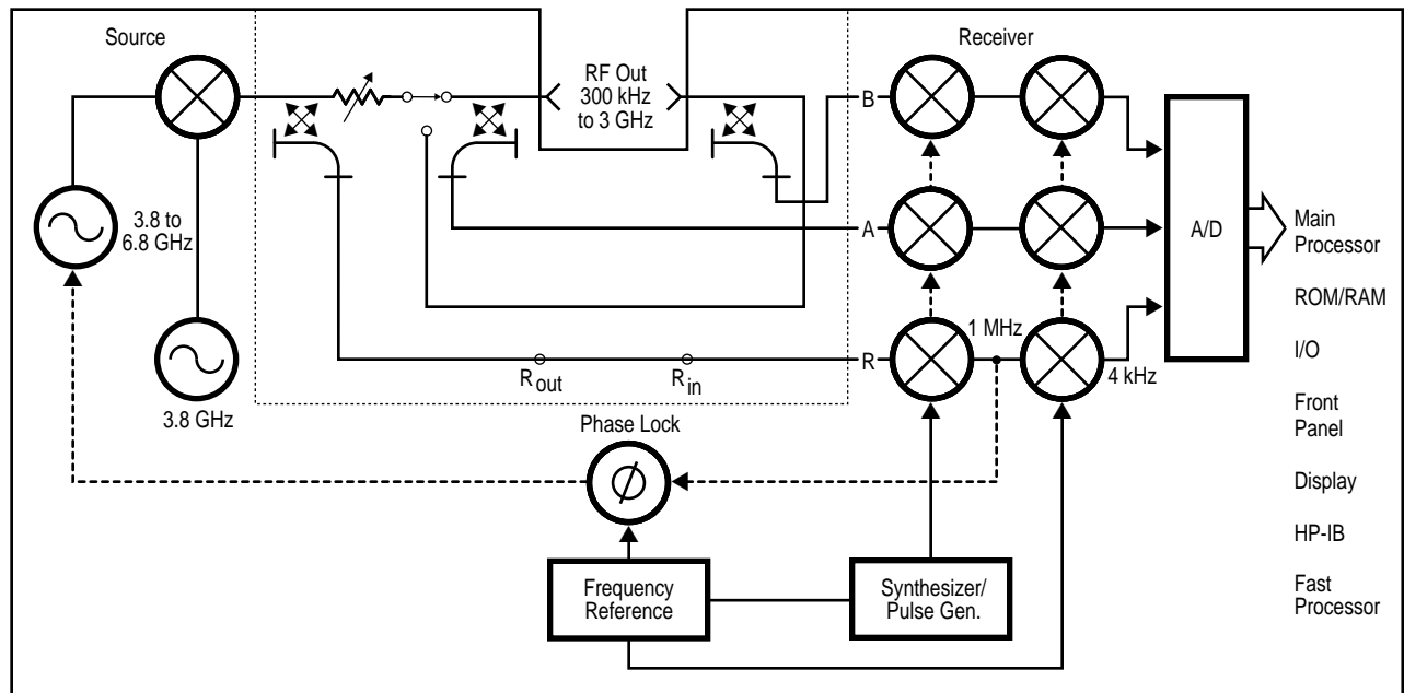
HP 8702D block diagram
