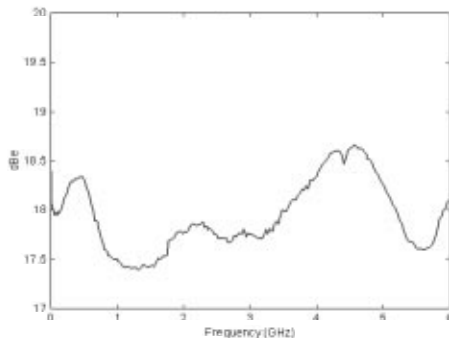
HP 83411D demodulation frequency response (characteristic)
