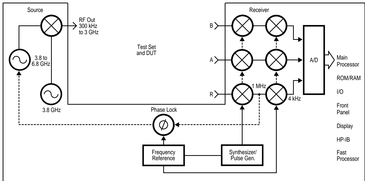
HP 8702D Option 011 block diagram
