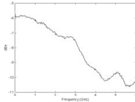
HP 83403C modulation frequency response (characteristic)
