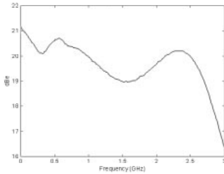
HP 83410C demodulation frequency response (characteristic)
