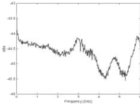
HP 83402B modulation frequency response (characteristic)
