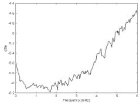
HP 83411C demodulation frequency response (characteristic)
