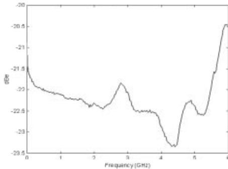
HP 83402A modulation frequency response (characteristic)
