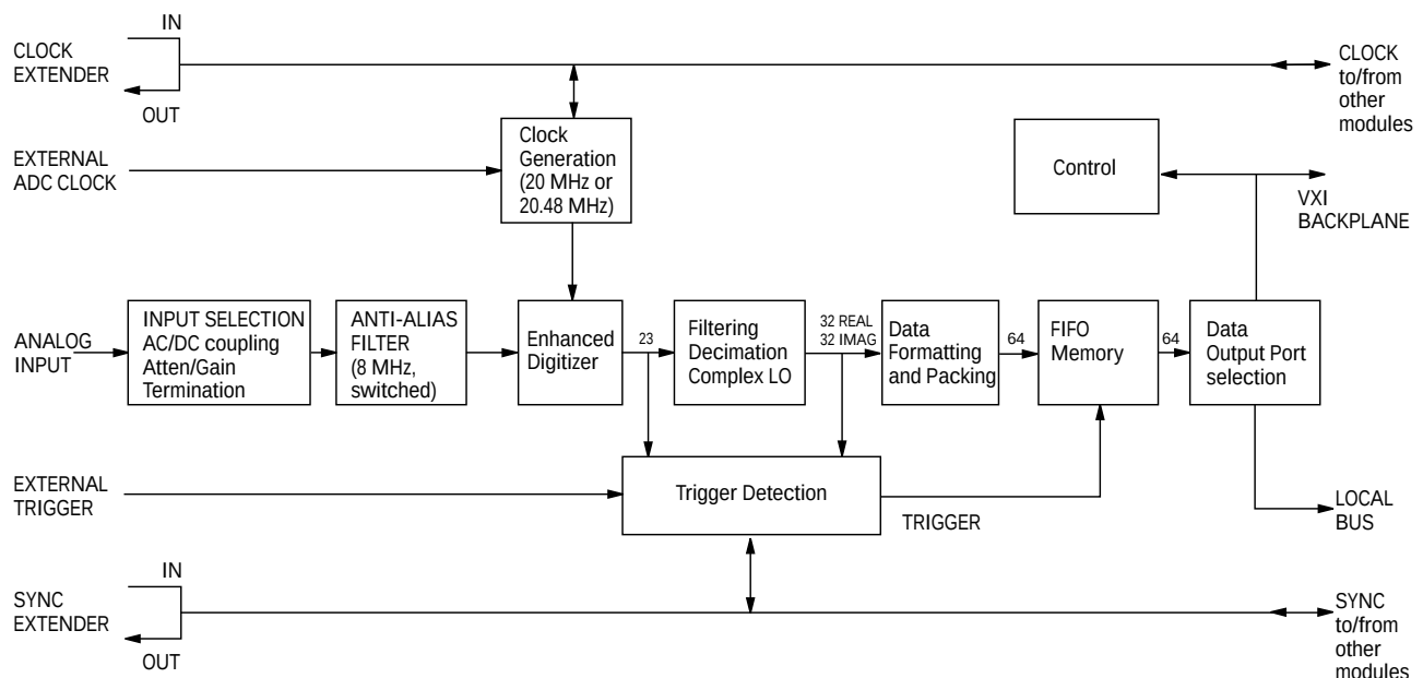
Figure 1: HP E1437A Block Diagram
