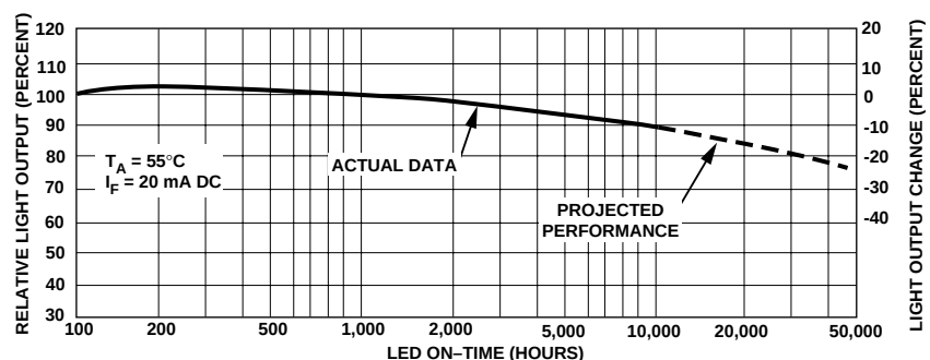
Figure 3. Statistical Average HTOL Light Output Degradation for Precision Optical Performance AlInGaP LED Lamps.
