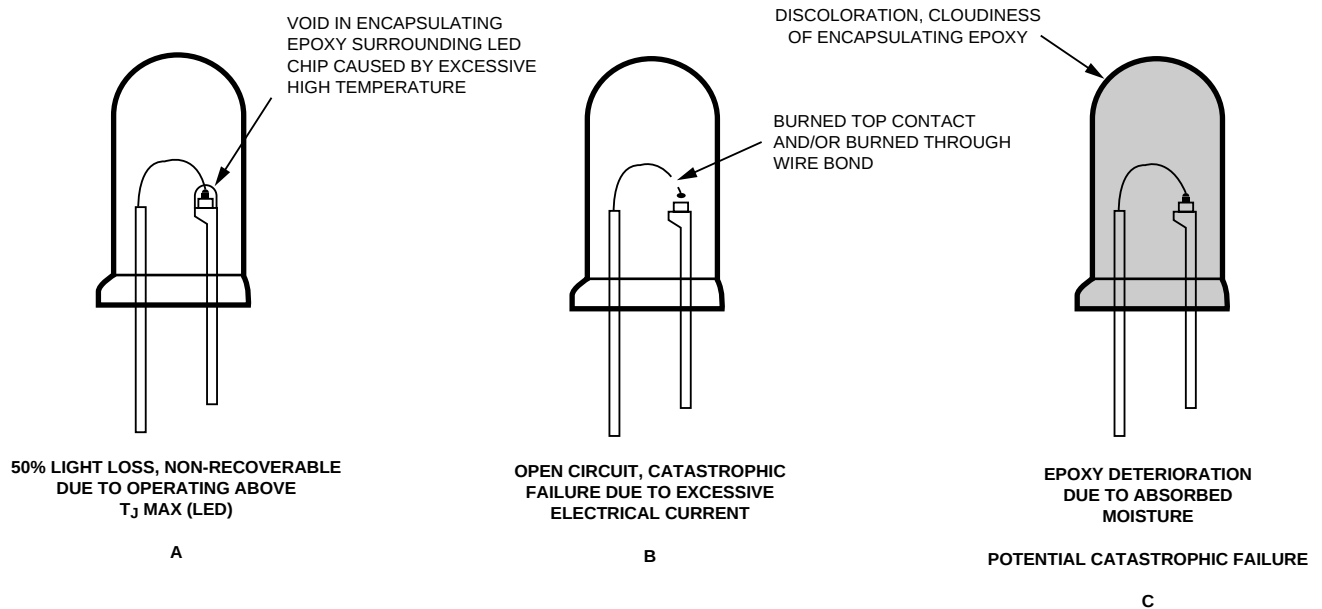
Figure 6. Typical LED Field Failure Modes That Can Occur with Excessive Current Drive or Inadequate Packaging Design.
