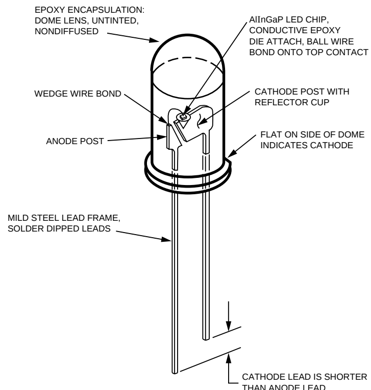
Figure 1. The Anatomy of a Precision Optical Performance AlInGaP LED T-13/4 Plastic Lamp.
