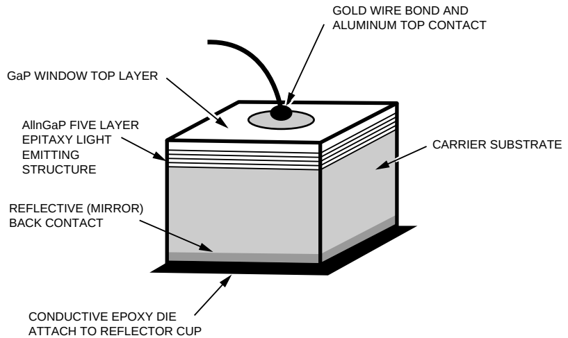
Figure 2. Details of an AlInGaP LED Chip.
