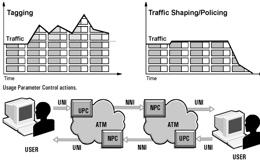
Usage Parameter Control (UPC) takes place between the user-equipment side and the network-equipment side of the UNI interface.
