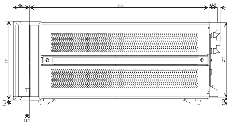
Figure 12. Agilent 4294A dimensions (side view, with Option 1CN/1D5, typical, in millimeters)
