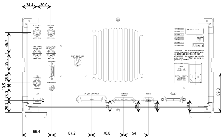
Figure 11. Agilent 4294A dimensions (rear view, with Option 1CN/1D5, typical, in millimeters)
