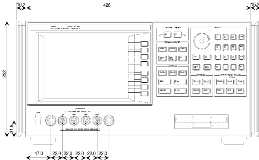
Figure 10. Agilent 4294A dimensions (front view, with Option 1CN/1D5, typical, in millimeters)
