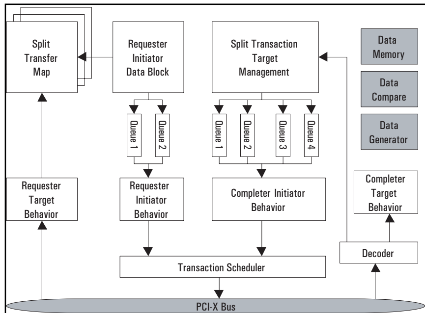
Figure 3: E2922A PCI-X exerciser architecture
