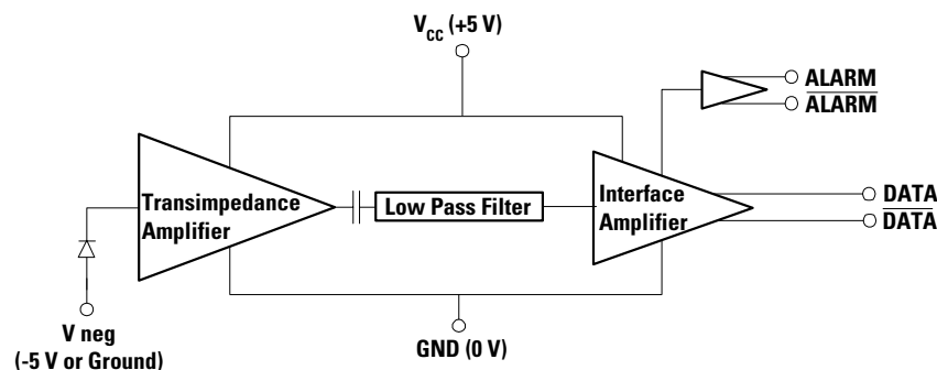
Figure 1. Block Diagram
