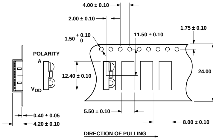
TAPE DIMENSIONS
