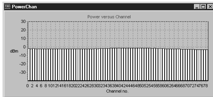
Figure 9. Agilent E1852A display showing a repartition of the power on the 79 Bluetooth channels.
