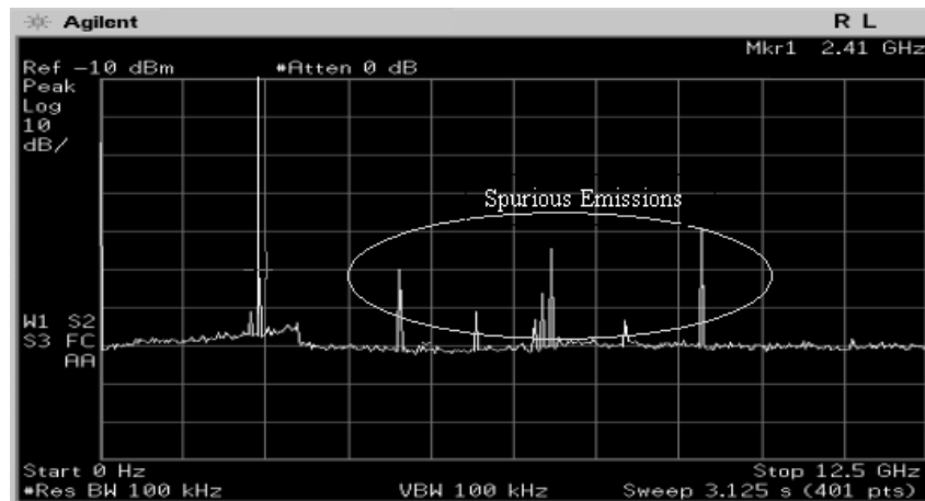
Figure 17. Agilent ESA-E spectrum analyzer display, showing a spurious analysis in the 12.5 GHz band.
