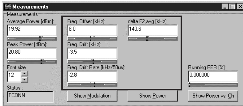
Figure 11. Agilent E1852A display showing the parameters ICFT (Frequency Offset), Frequency Deviation, and Frequency Drift which you should analyze.
