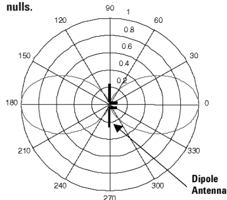
Figure 18. Example of a radiation pattern diagram: A polar diagram of a dipole antenna showing area with low gain or nulls.
