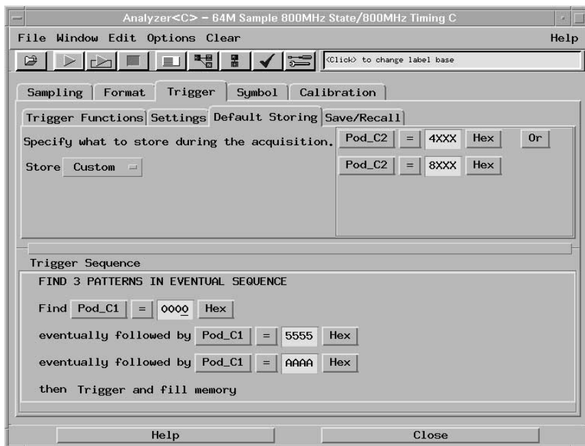
Figure 7. Find patterns in eventual sequence with custom store qualification
