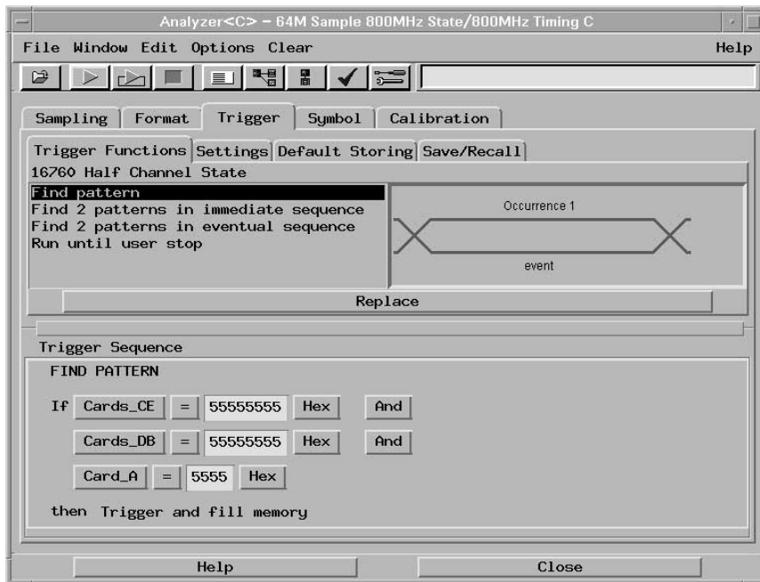
Figure 9. An analyzer-wide pattern on a 5-card module using 32-bit split labels
