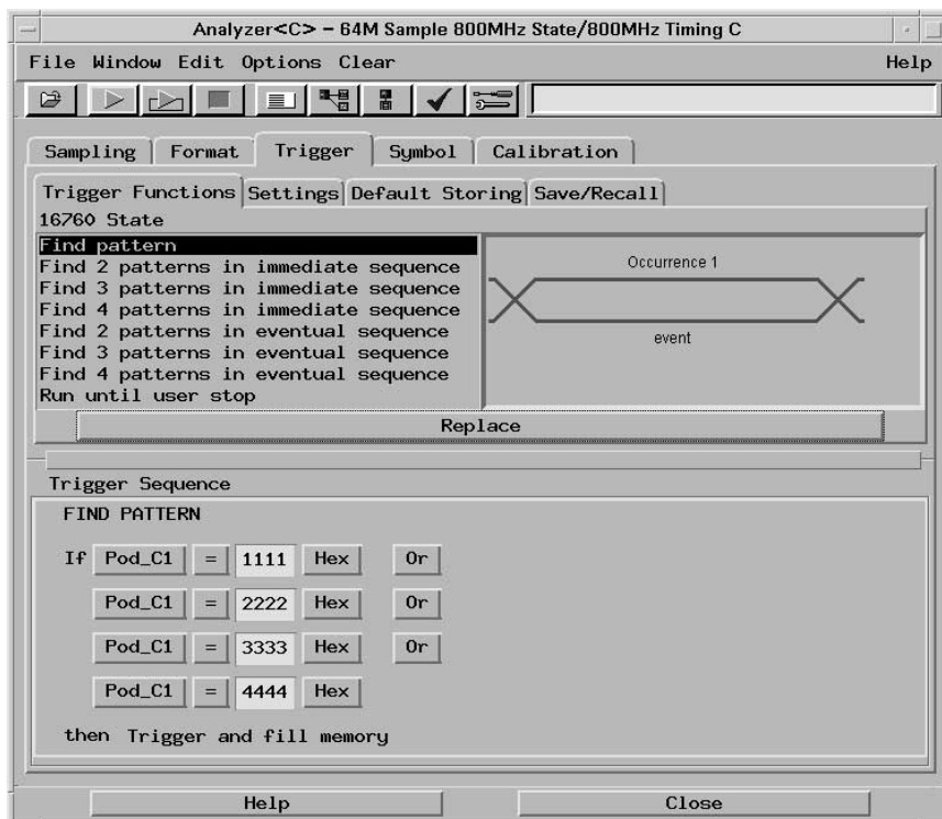
Figure 2. Find 4 patterns on a single pod.
