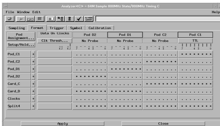
Figure 8. In half channel state mode, it takes a minimum of 4 pods (at 8 bits per pod) to fill a 32 bit split label as shown by label 'Split4'.
