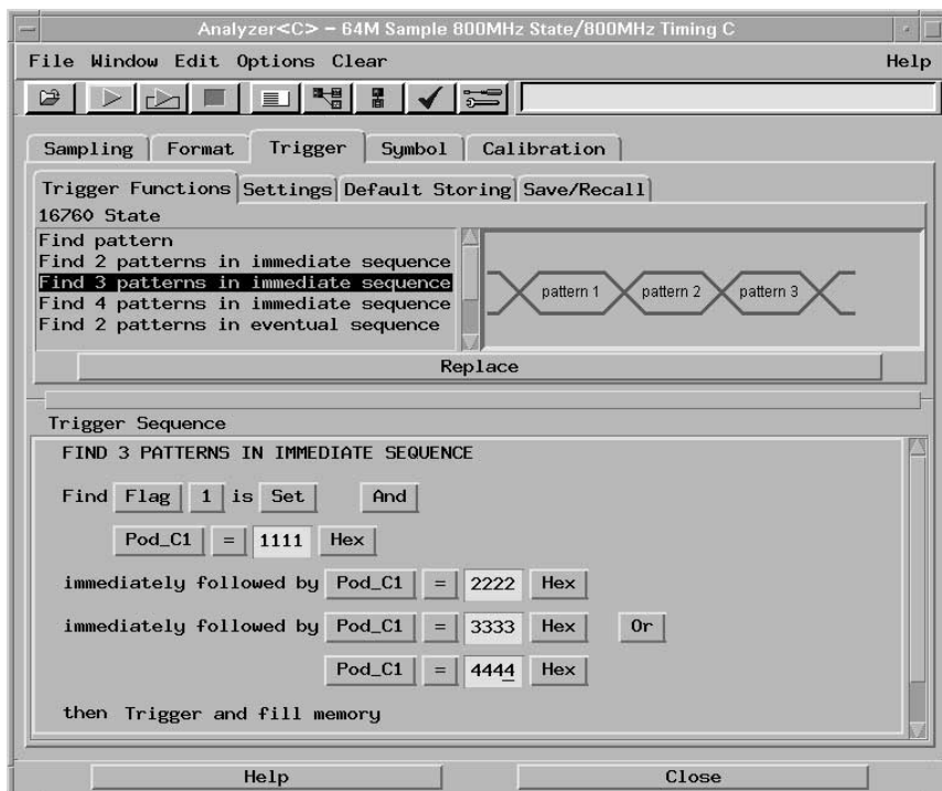
Figure 6. Using 4 patterns in 3 sequence levels.
