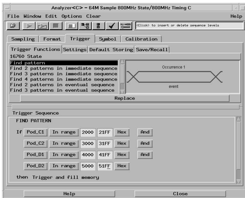
Figure 5. A Multiple ranges
