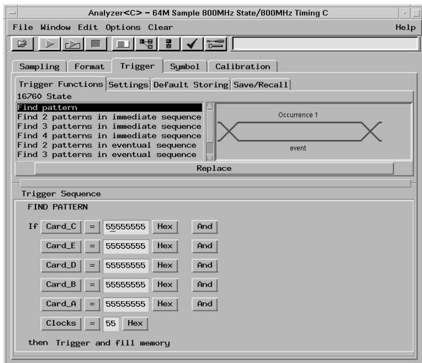
Figure 3. Find a single pattern across the entire analyzer in a 5-card set.
