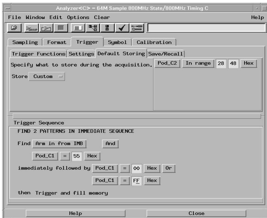
Figure 11. An Arm in from IMB in a Find 2 patterns in immediate sequence trigger function
