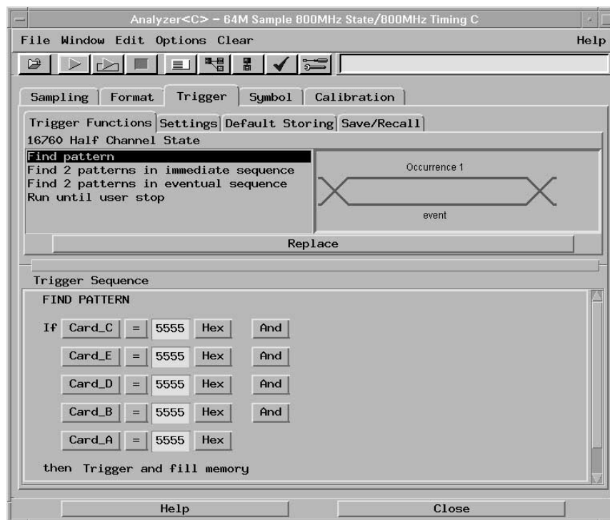
Figure 10. An analyzer-wide pattern on a 5-card module using 16-bit split labels.
