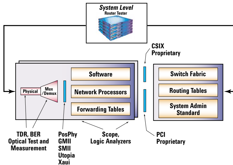
Figure 15. Router system triggering
