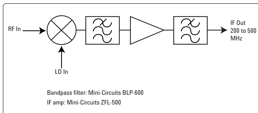
Figure 13. Block diagram of suggested downconverter. See Table 4 for further details.
