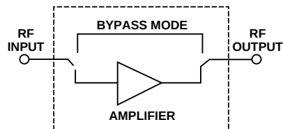
Figure 1. MGA-72543 Functional Diagram.
