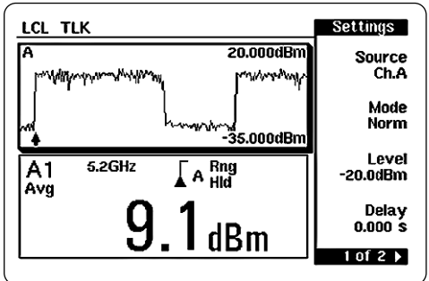
Figure 9: Average power measurement of IEEE 802.11a, using EPM-P
