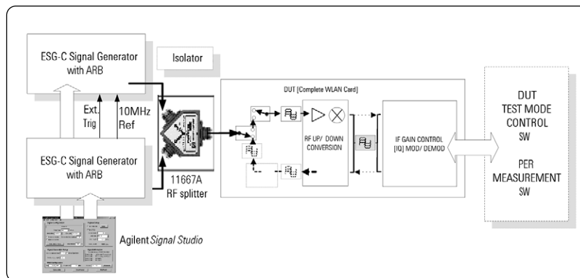
Figure 29: Test configuration for receiver adjacent channel and blocking tests
