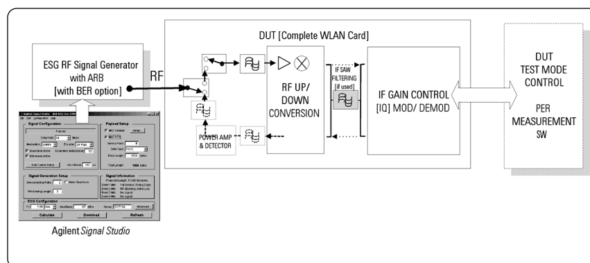
Figure 28: Diagram of complete receiver measurement path
