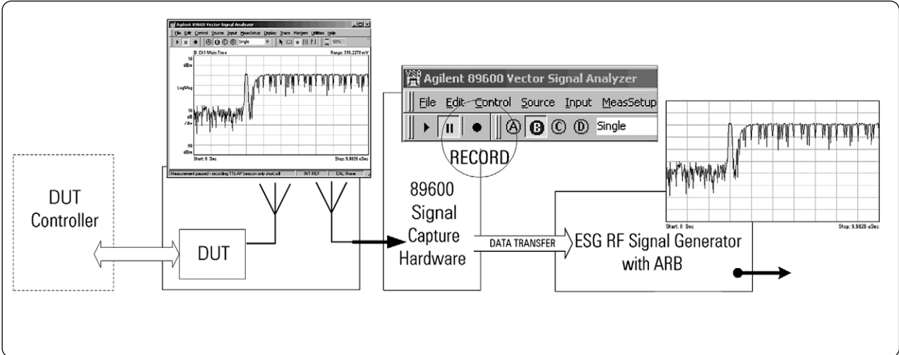
Figure 24: Signal record/replay of suspect signal using Agilent 89600 Vector Signal Analyzer and ESG
