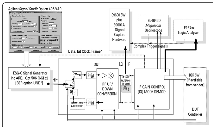
Figure 27: Diagram of analog-only receiver measurement paths
