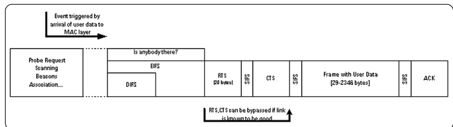
Figure 6a: Outline process to send data (IEEE 802.11)
