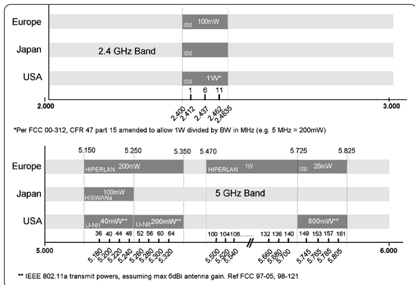
Figure 1: Major channel allocations and power levels
