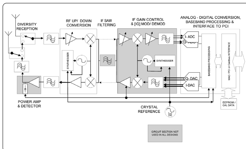
Figure 2: Block diagram of a WLAN card
