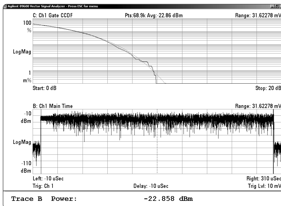
Figure 10: Combined display plot, including IEEE 802.11a CCDF measurement
