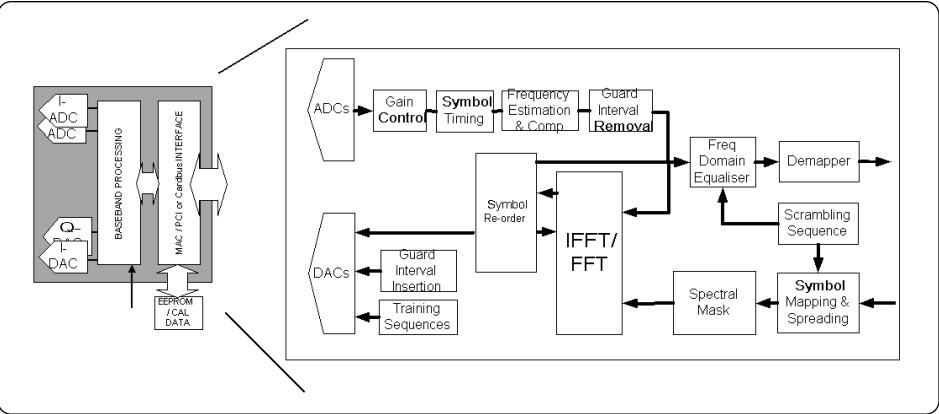
Figure 3: Digital processing blocks for an OFDM transceiver
