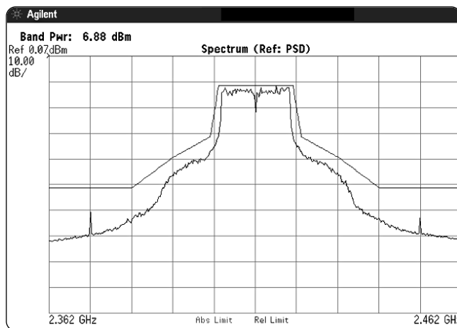
Figure 12: IEEE 802.11a signal measured using Agilent performance spectrum analyzer
