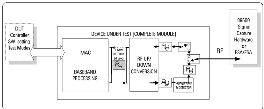
Figure 8: Transmitter test configuration for a complete WLAN card
