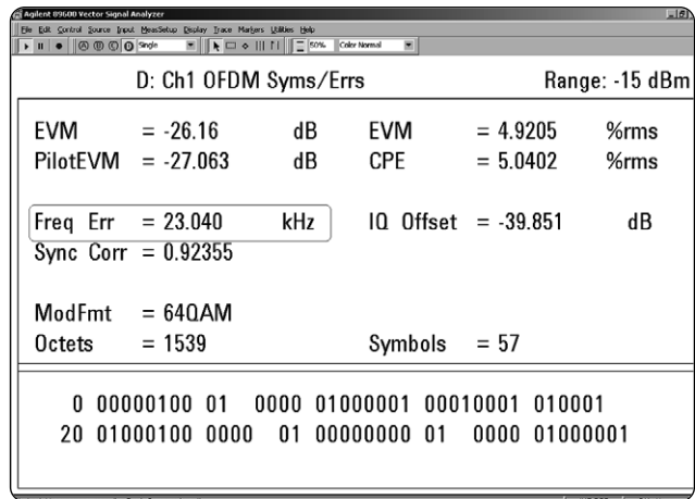
Figure 19a: Frequency error from an IEEE 802.11a device
