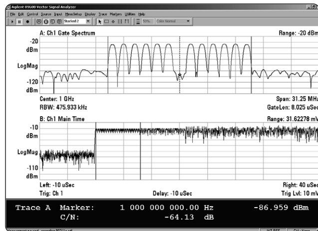
Figure 14: Plot showing center frequency leakage of an IEEE 802.11a signal
