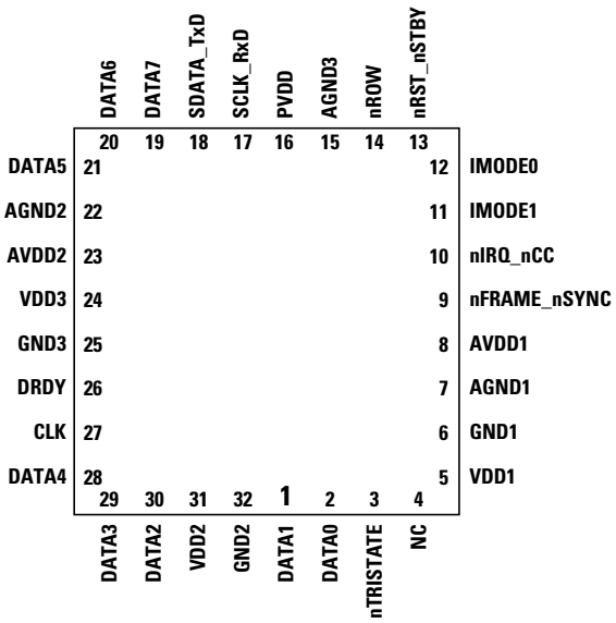
ADCS-1021 32 Pin Package Diagram
