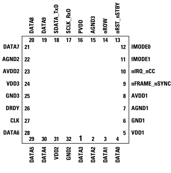
ADCS-2021 32 Pin Package Diagram
