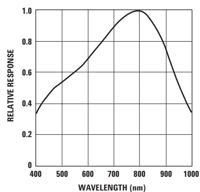
Figure 17. Wavelength Responsivity [1] .
