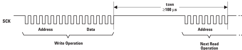
Figure 27. Timing between write and read commands.
