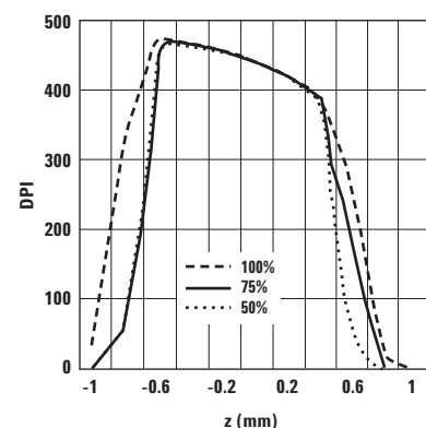
Figure 18. Typical Resolution vs. Height at different LED current levels on manila folder.
