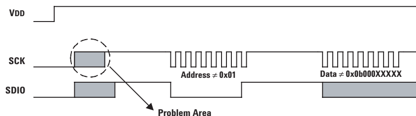
Figure 29. Power-up serial port sequence.
