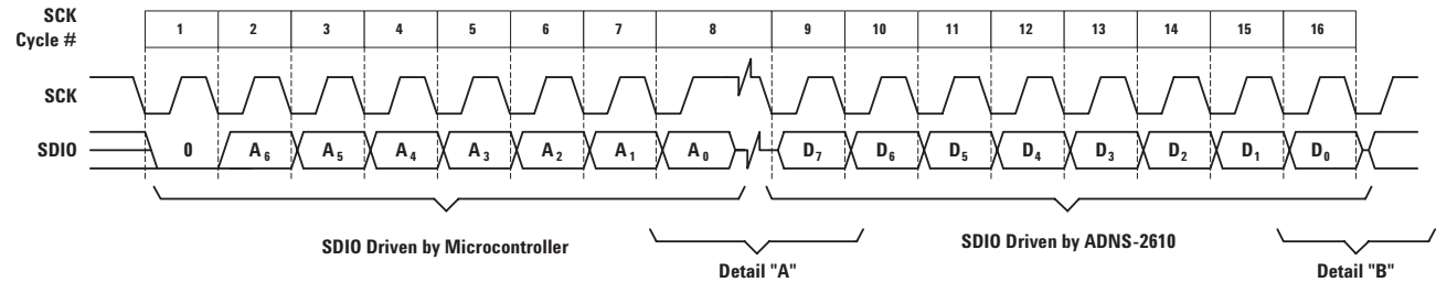
Figure 22. Read operation.
