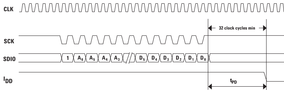
Figure 13. Power-down timing.
