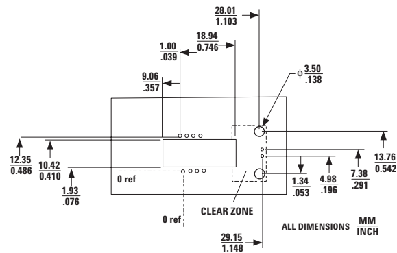
Figure 3. Recommended PCB mechanical cutouts and spacing.
