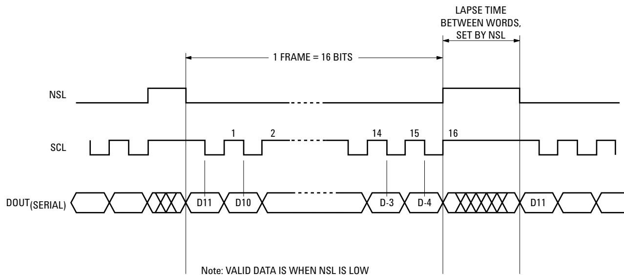
Figure 2. Timing diagram.
